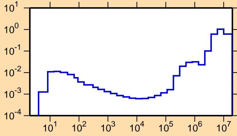
\sigma vs. E for ^{193}\text{Bi}(n,\text{inel.})
