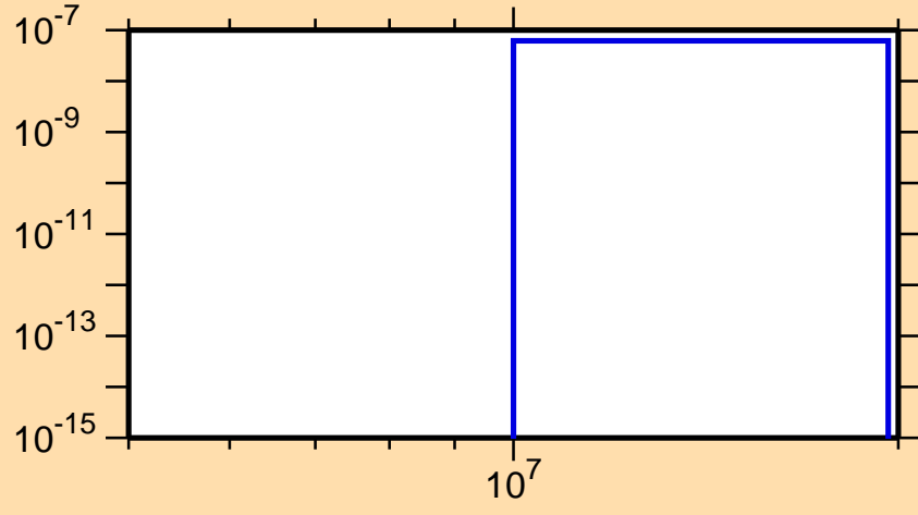
\sigma vs. E for ^{193}\text{Bi}(n,nd)
