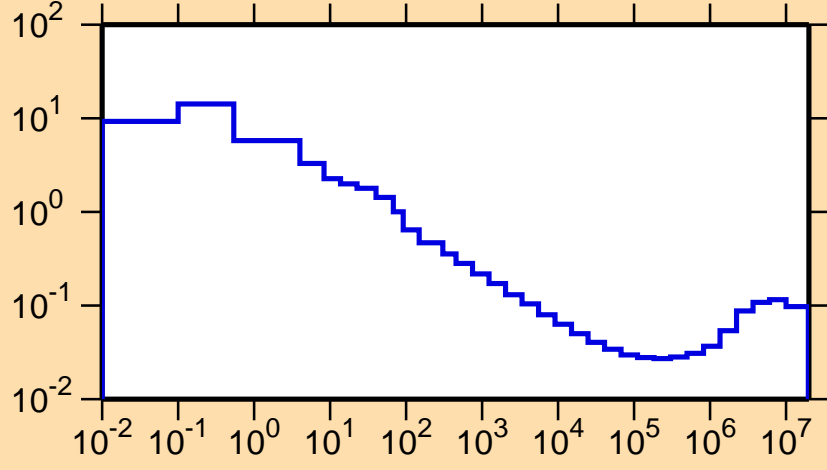
\sigma vs. E for ^{193}\text{Bi}(n,p)
