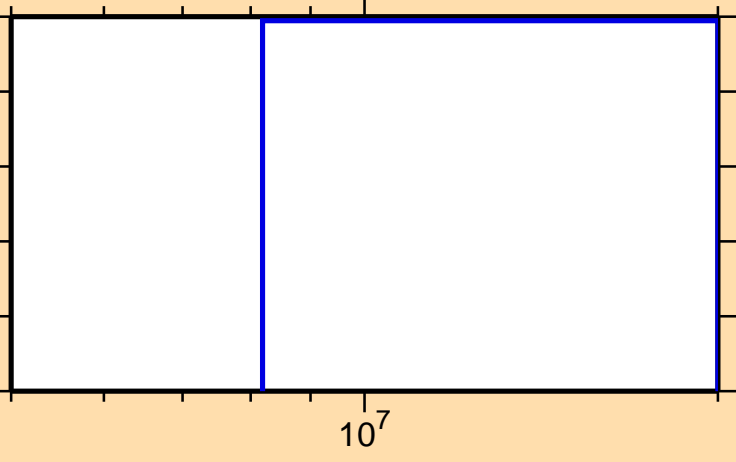
\sigma vs. E for ^{193}\text{Bi}(\text{mt117})
