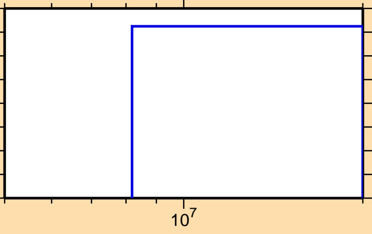
\sigma vs. E for ^{193}\text{Bi}(n,3n)
