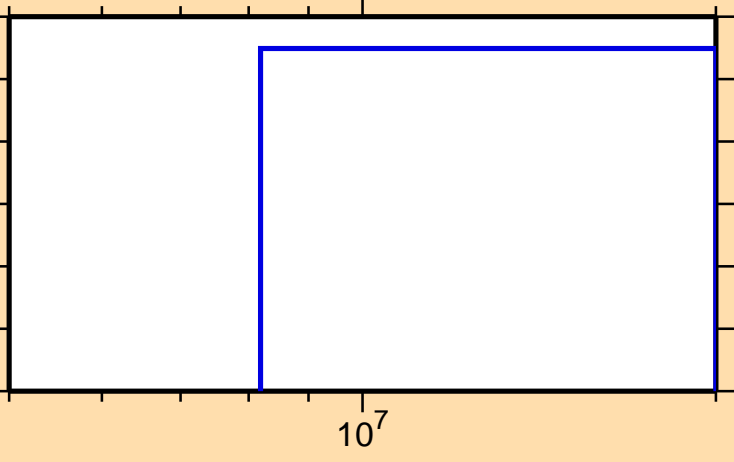
\sigma vs. E for ^{193}\text{Bi}(n,\text{pd})
