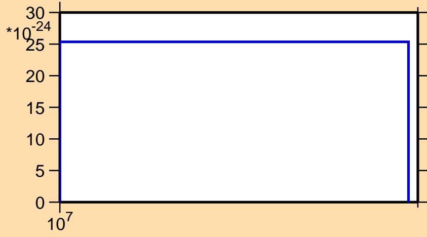
\sigma vs. E for ^{194}\text{Bi} (mt 42)
