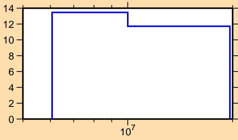
\Delta\sigma/\sigma vs. E for ^{194}\text{Bi}(n,\text{nonel.})
