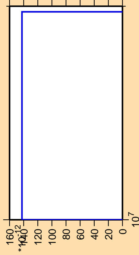
\Delta\sigma/\sigma vs. E for ^{194}\text{Bi} (mt 42)
