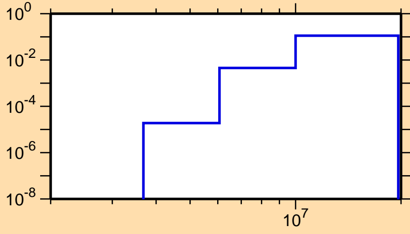
\sigma vs. E for ^{194}\text{Bi}(n,np)
