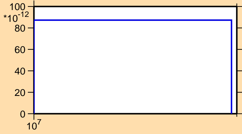
\sigma vs. E for ^{194}\text{Bi}(n,nt)
