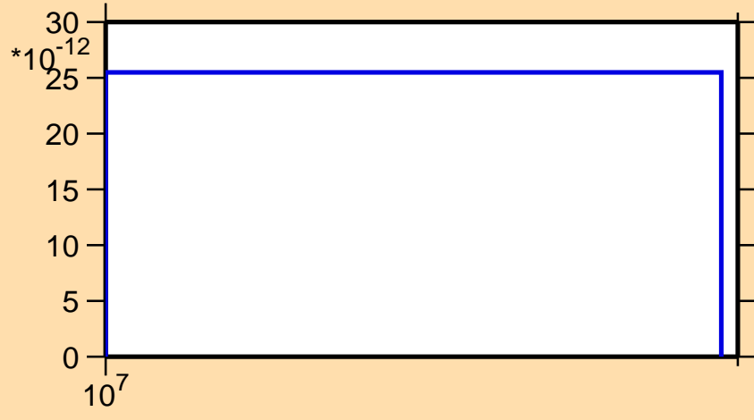
\sigma vs. E for ^{194}\text{Bi} (mt 34)
