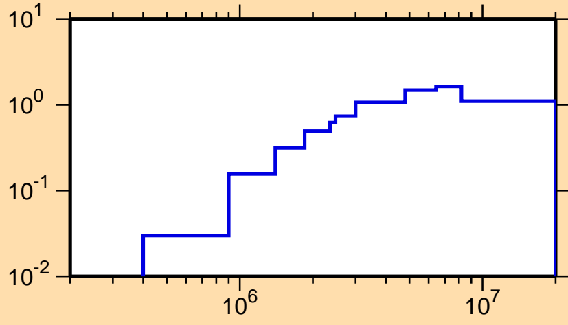
\sigma vs. E for ^{194}\text{Bi}(n,\text{inel.})
