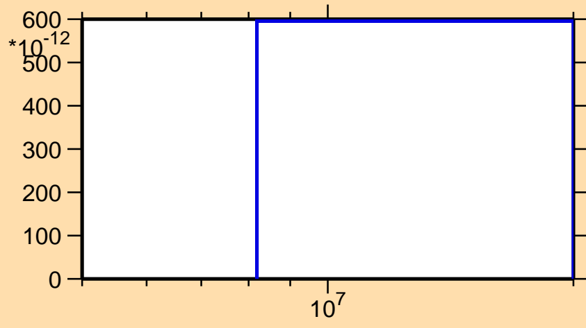
\sigma vs. E for ^{194}\text{Bi}(\text{mt117})
