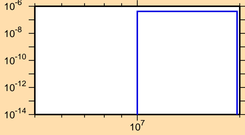
\sigma vs. E for ^{194}\text{Bi}(n,nd)
