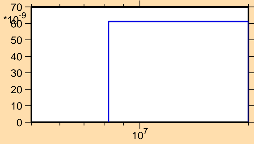
\sigma vs. E for ^{194}\text{Bi} (mt 45)
