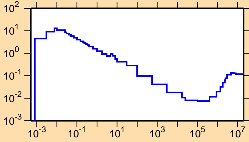
\sigma vs. E for ^{194}\text{Bi}(n,p)
