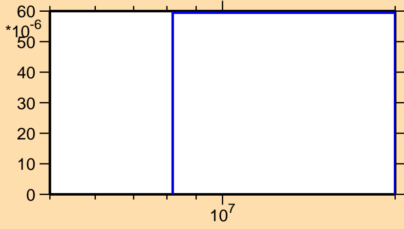
\sigma vs. E for ^{194}\text{Bi}(n,2np)
