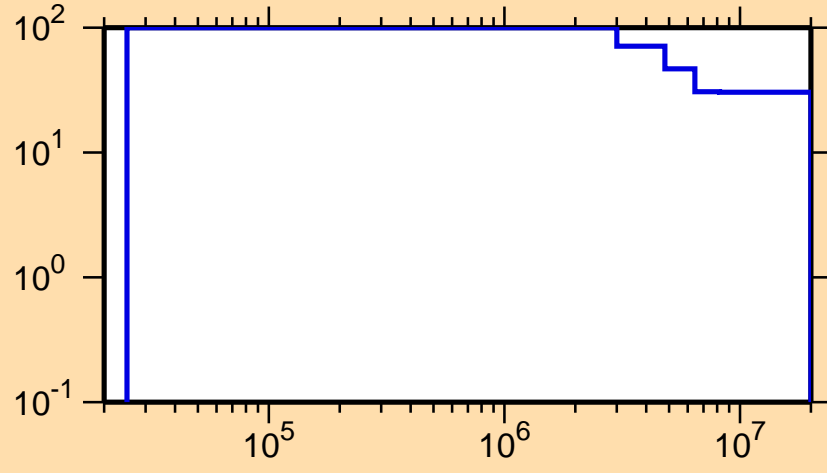
\Delta\sigma/\sigma vs. E for ^{194}\text{Bi}(n,n\text{cont.})
