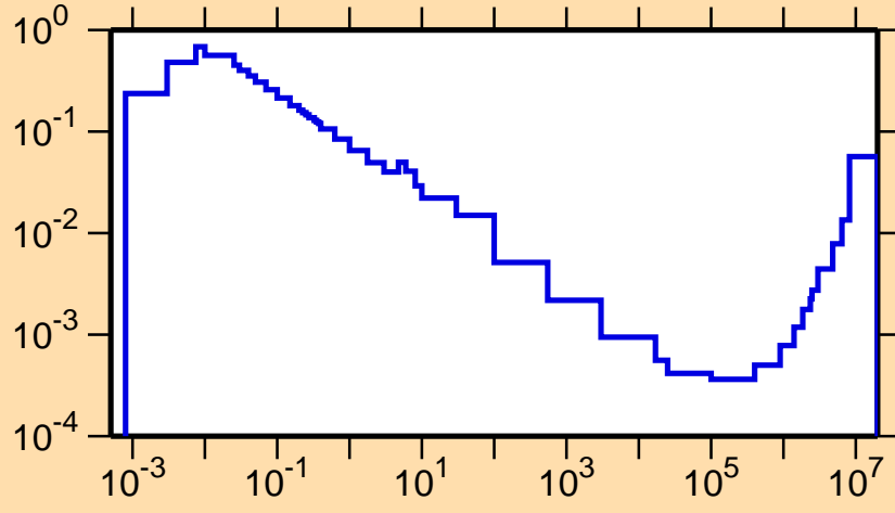
\sigma vs. E for ^{194}\text{Bi}(n,\alpha)
