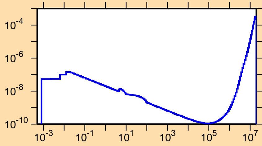
\sigma vs. E for ^{194}\text{Bi}(n,p\alpha)
