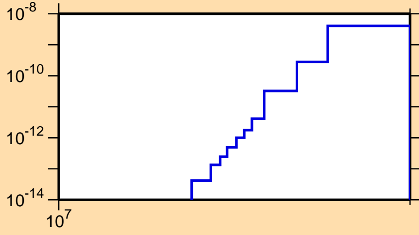
\sigma vs. E for ^{194}\text{Bi} (mt 34)
