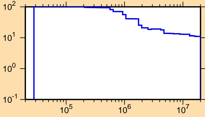
\Delta\sigma/\sigma vs. E for ^{194}\text{Bi}(n,n\text{nonel.})
