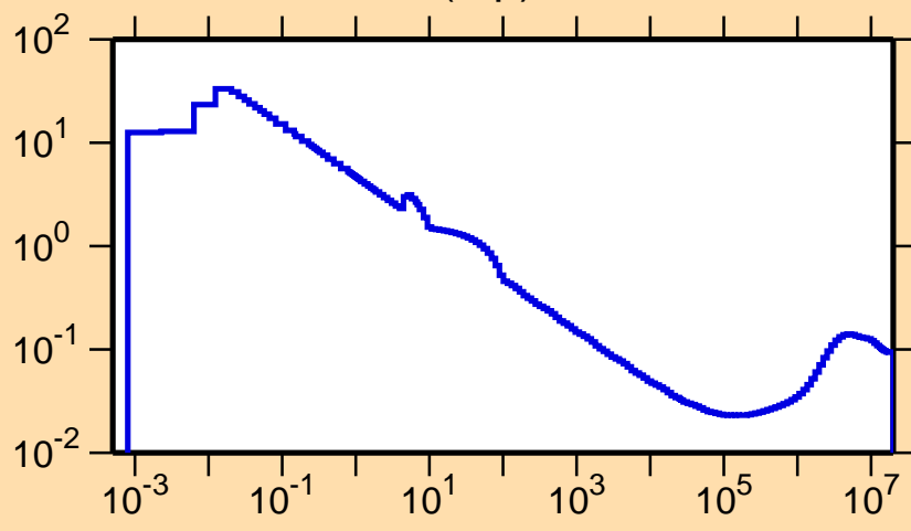
\sigma vs. E for ^{194}\text{Bi}(n,p)
