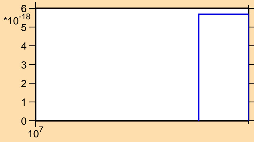
\sigma vs. E for ^{194}\text{Bi} (mt 42)
