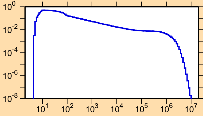
\sigma vs. E for ^{194}\text{Bi}(n,n_1)
