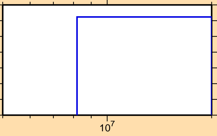
\sigma vs. E for ^{194}\text{Bi}(n,3n)
