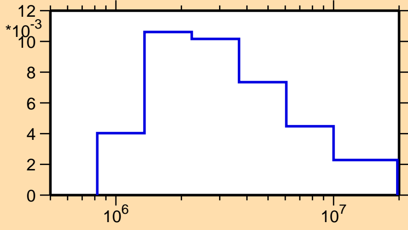
\sigma vs. E for ^{195}\text{Bi}(n,n_2)
