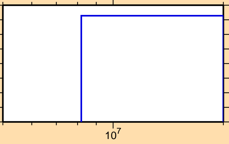
\sigma vs. E for ^{195}\text{Bi}(n,3n\alpha)
