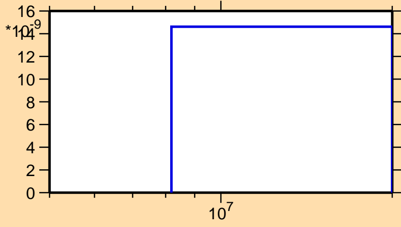
\sigma vs. E for ^{195}\text{Bi} (mt 45)
