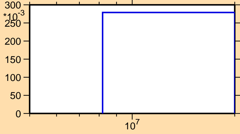
\sigma vs. E for ^{195}\text{Bi}(n,2n)
