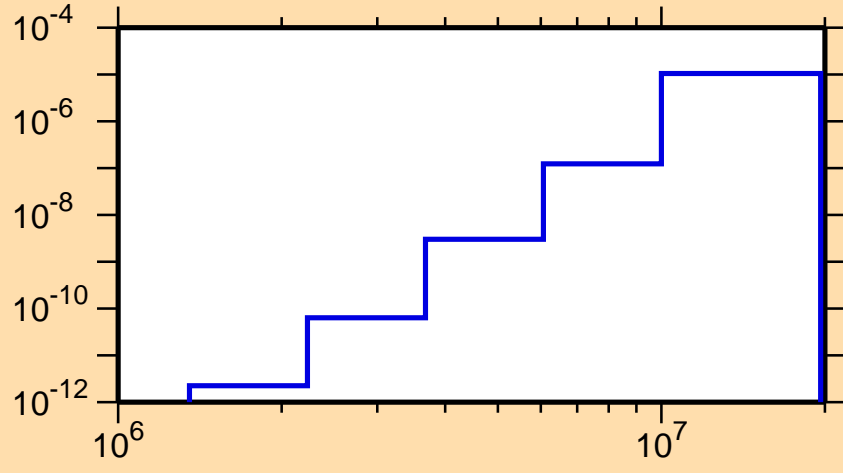
\sigma vs. E for ^{195}\text{Bi}(n,p\alpha)
