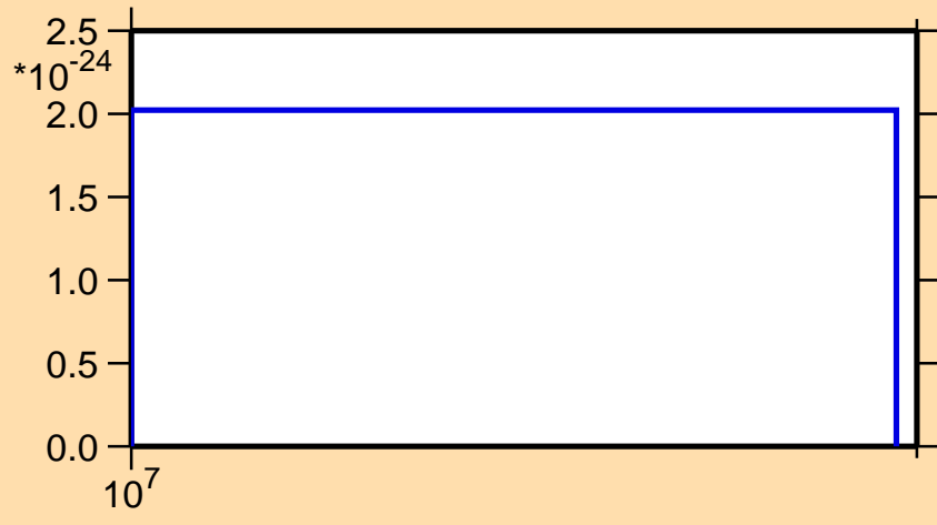
\sigma vs. E for ^{195}\text{Bi} (mt 42)
