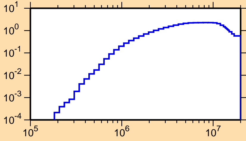
\sigma vs. E for ^{196}\text{Bi}(n,\text{inel.})
