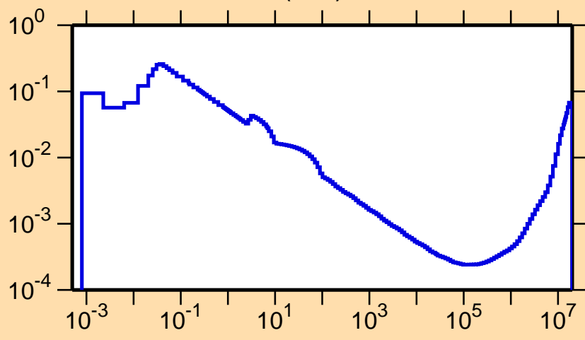
\sigma vs. E for ^{196}\text{Bi}(n,\alpha)
