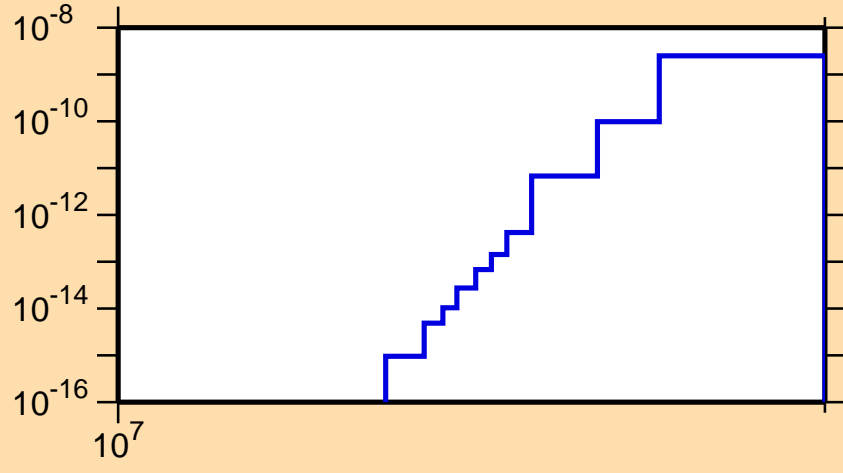
\sigma vs. E for ^{196}\text{Bi}(n,\text{pt})
