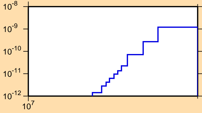
\sigma vs. E for ^{196}\text{Bi}(\text{mt117})
