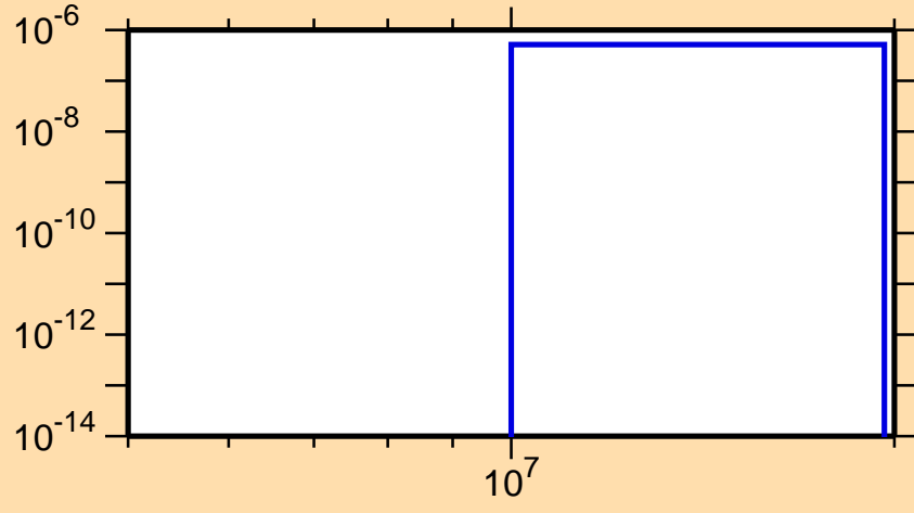
\sigma vs. E for ^{196}\text{Bi}(n,nd)
