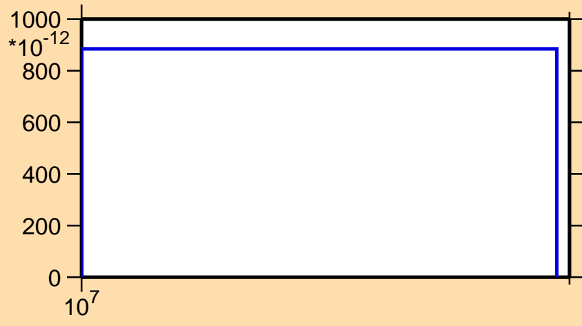
\sigma vs. E for ^{196}\text{Bi}(n,\text{pd})
