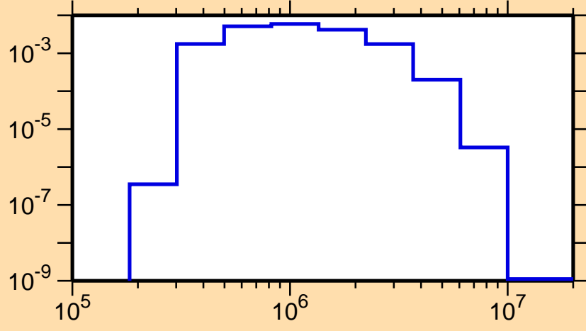
\sigma vs. E for ^{196}\text{Bi}(n,n_4)
