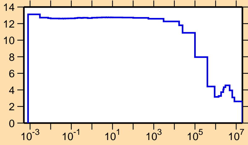
\sigma vs. E for ^{196}\text{Bi}(n,\text{el.})
