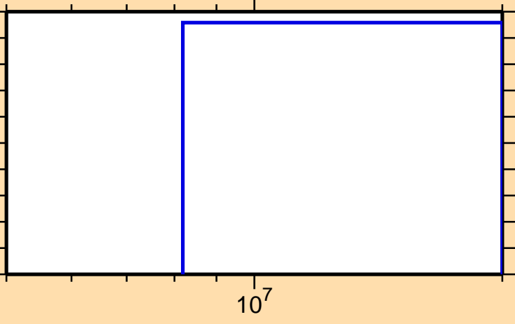
\sigma vs. E for ^{196}\text{Bi}(n,nt)
