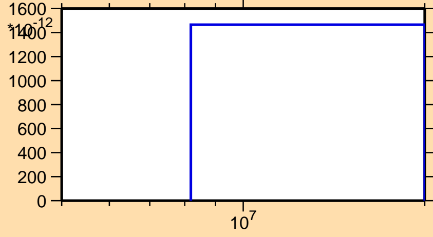
\sigma vs. E for ^{196}\text{Bi} (mt 45)
