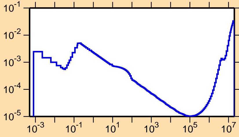
\sigma vs. E for ^{197}\text{Bi}(n,\alpha)
