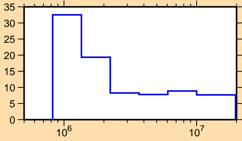
\Delta\sigma/\sigma vs. E for ^{197}\text{Bi}(n,n\text{onel.})
