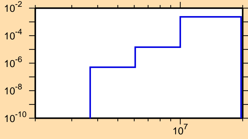
\sigma vs. E for ^{197}\text{Bi}(n,n\alpha)
