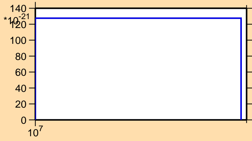
\sigma vs. E for ^{197}\text{Bi} (mt 42)
