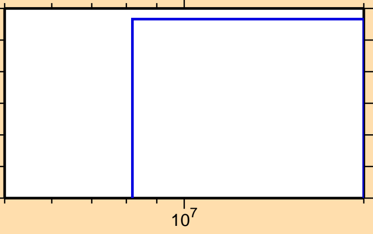
\sigma vs. E for ^{197}\text{Bi}(n,3n)
