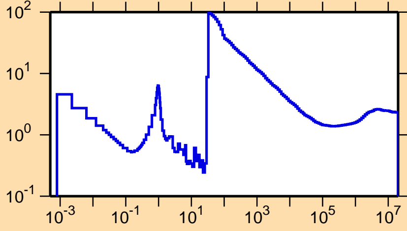
\sigma vs. E for ^{197}\text{Bi}(n,\text{nonel.})
