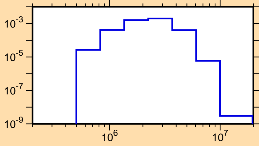
\sigma vs. E for ^{197}\text{Bi}(n,n_2)
