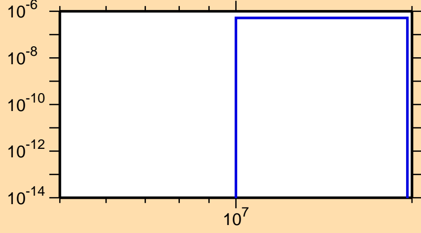
\sigma vs. E for ^{198}\text{Bi}(n,nd)
