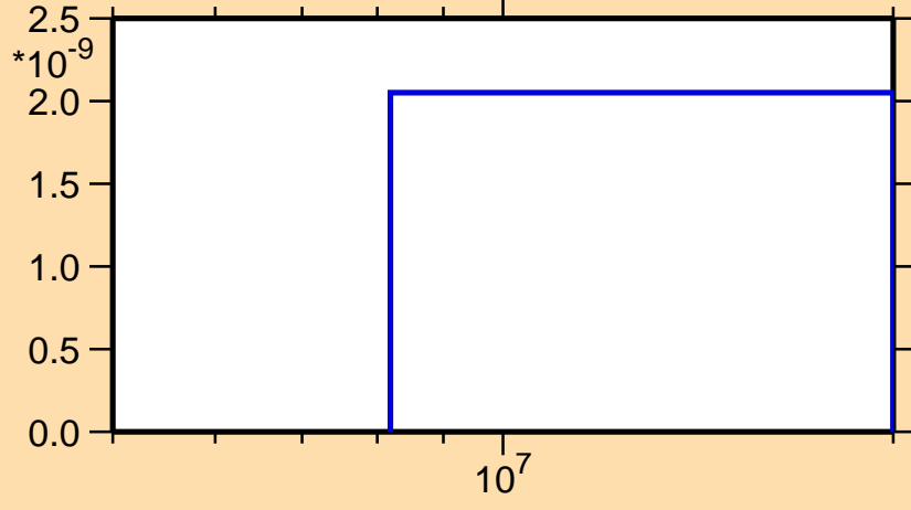
\sigma vs. E for ^{198}\text{Bi}(n,nt)
