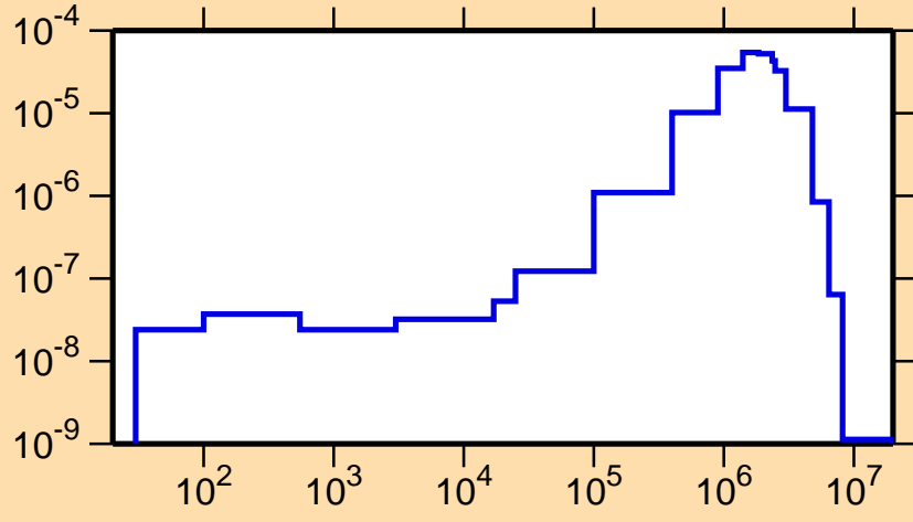
\sigma vs. E for ^{198}\text{Bi}(n,n_2)
