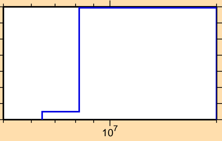
\sigma vs. E for ^{198}\text{Bi}(n,\text{He3})
