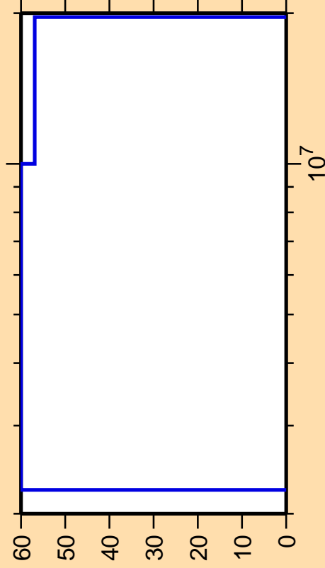
\Delta\sigma/\sigma vs. E for ^{198}\text{Bi}(n,np)
