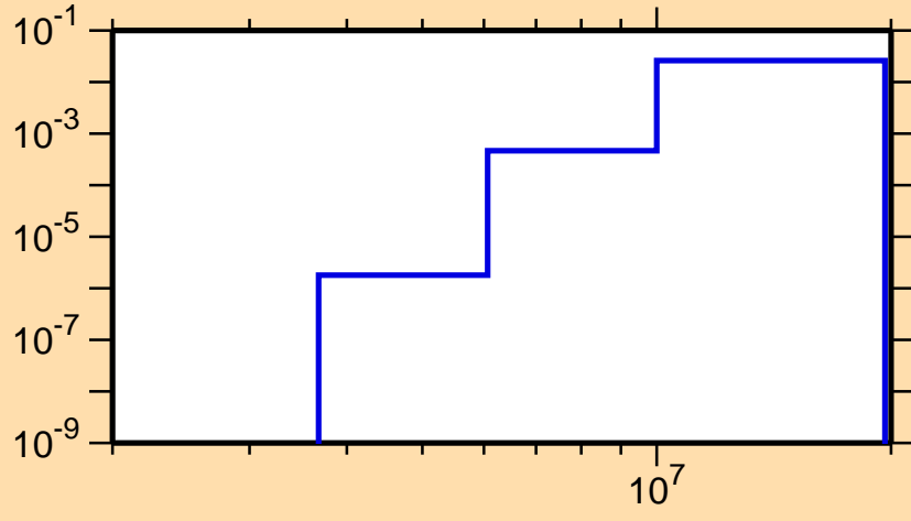
\sigma vs. E for ^{198}\text{Bi}(n,np)
