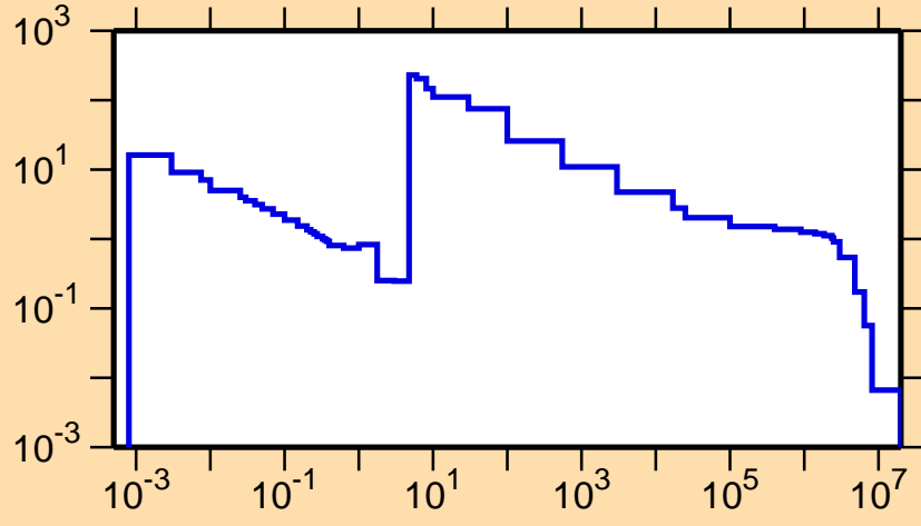
\sigma vs. E for ^{198}\text{Bi}(n,\gamma)
