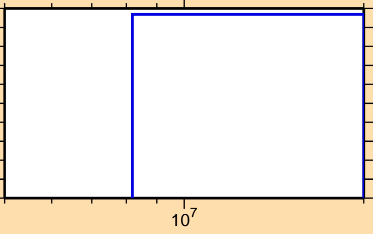
\sigma vs. E for ^{198}\text{Bi}(n,nt)
