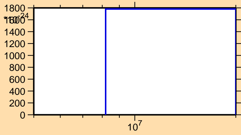
\sigma vs. E for ^{198}\text{Bi} (mt 42)
