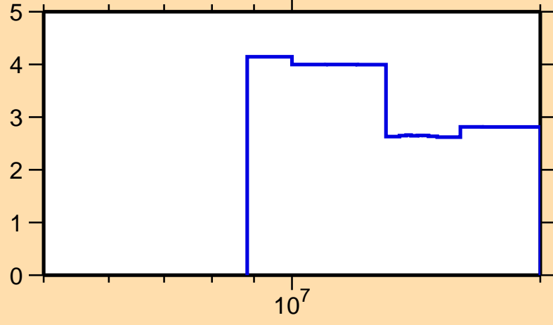
\Delta\sigma/\sigma vs. E for ^{199}\text{Bi}(n,\text{tot.})
