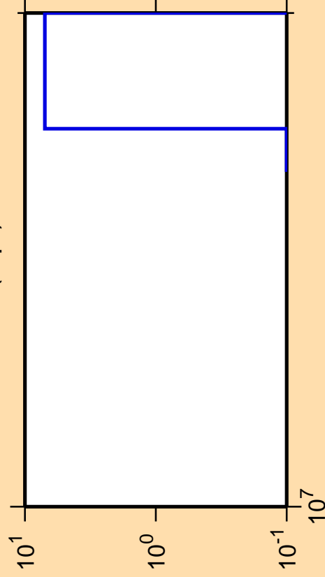
\Delta\sigma/\sigma vs. E for ^{199}\text{Bi}(n,\text{pt})
