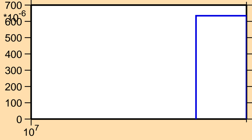
\sigma vs. E for ^{199}\text{Bi}(n,3n)
