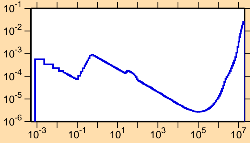
\sigma vs. E for ^{199}\text{Bi}(n,\alpha)
