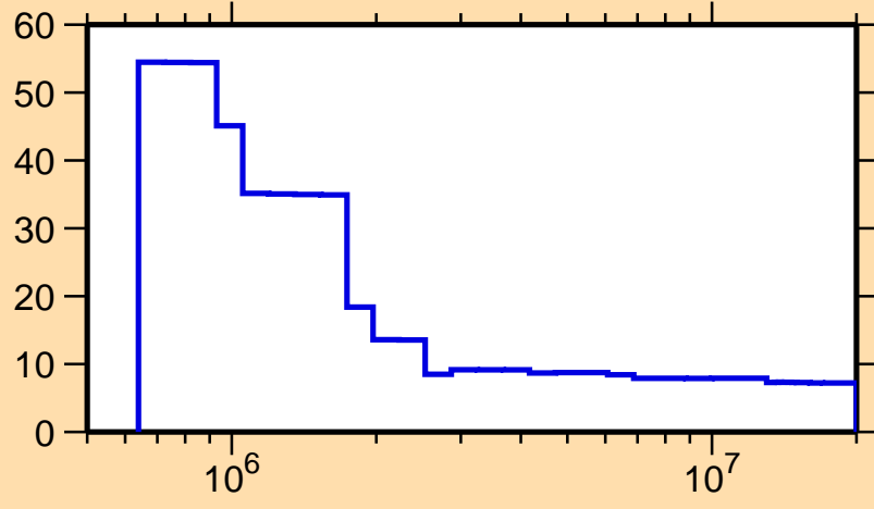
\Delta\sigma/\sigma vs. E for ^{199}\text{Bi}(n,\text{nonel.})
