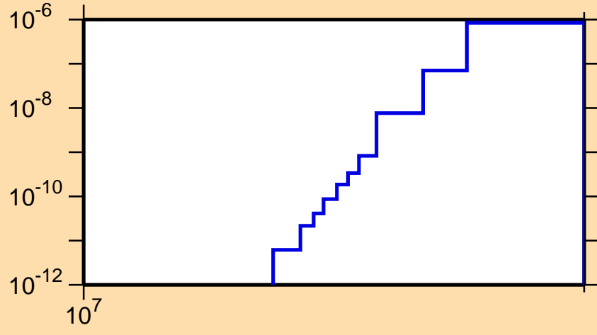
\sigma vs. E for ^{199}\text{Bi}(n,2n\alpha)
