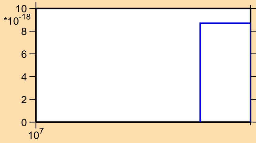
\sigma vs. E for ^{199}\text{Bi} (mt 42)
