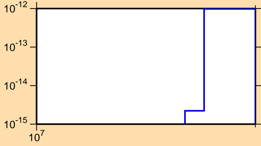
\sigma vs. E for ^{199}\text{Bi}(n,\text{pt})
