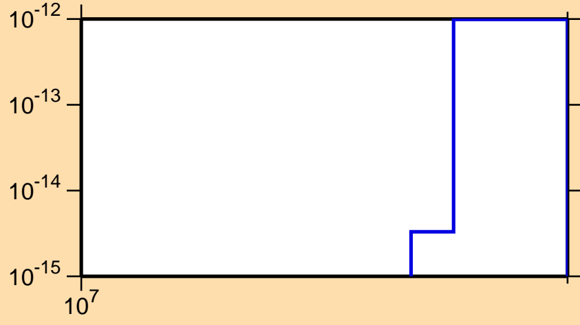
\sigma vs. E for ^{199}\text{Bi} (mt 34)
