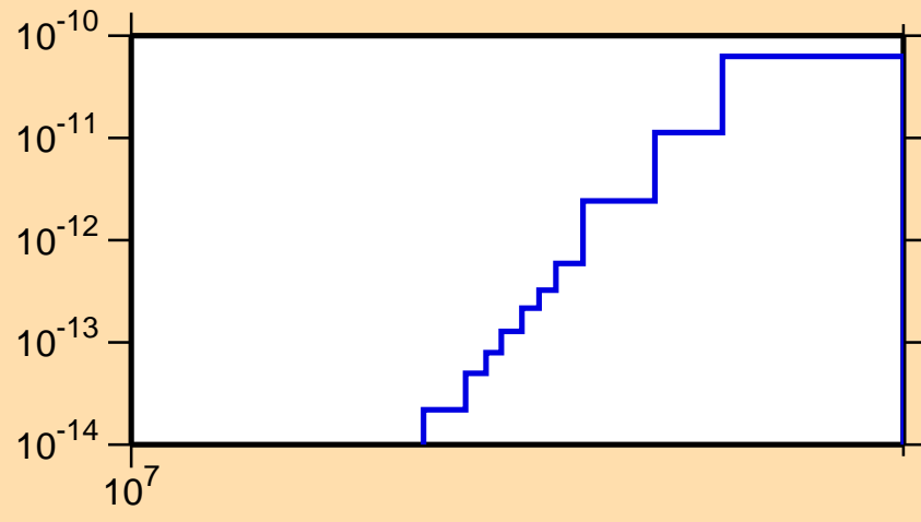
\sigma vs. E for ^{199}\text{Bi}(\text{mt117})
