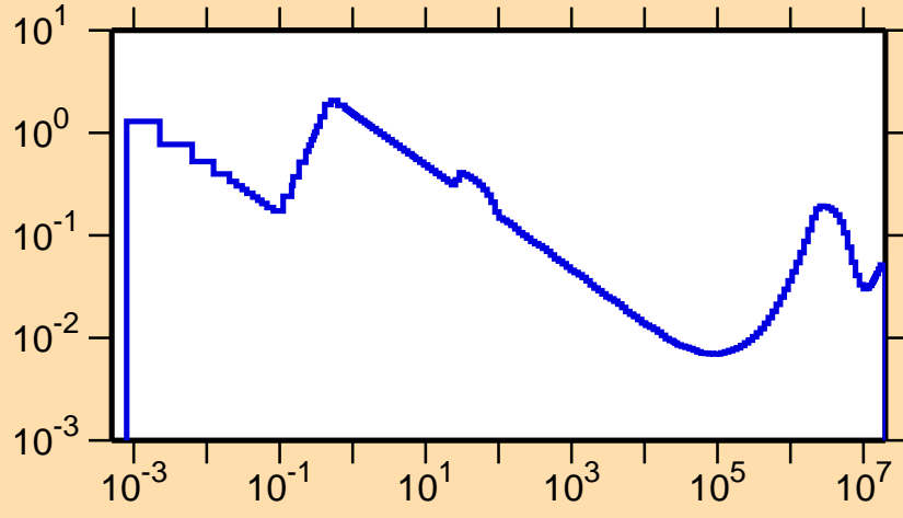
\sigma vs. E for ^{199}\text{Bi}(n,p)
