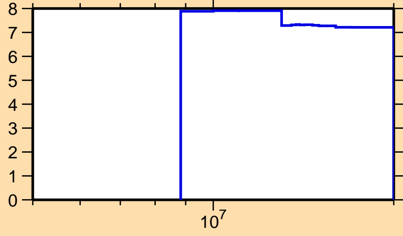
\Delta\sigma/\sigma vs. E for ^{199}\text{Bi}(n,\text{nonel.})
