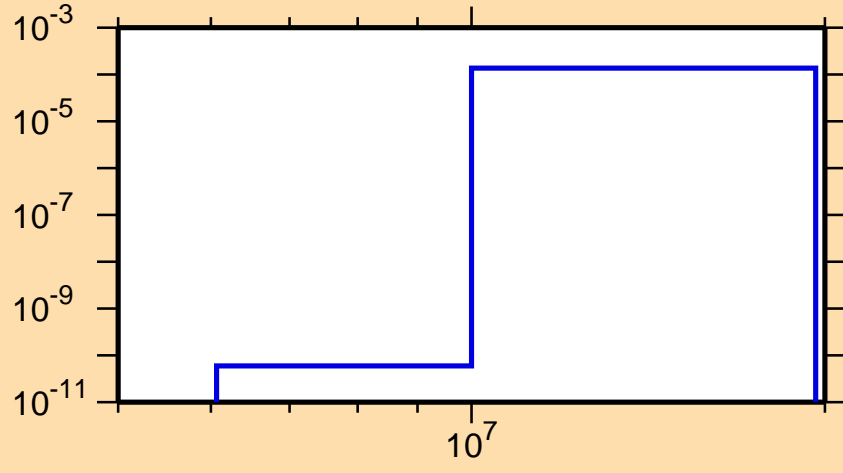
\sigma vs. E for ^{199}\text{Bi}(n,t)
