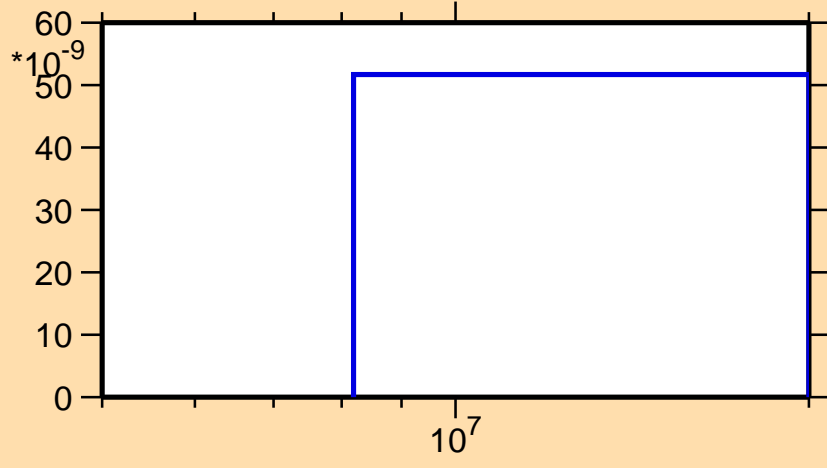
\sigma vs. E for ^{199}\text{Bi}(n,\text{He}3)
