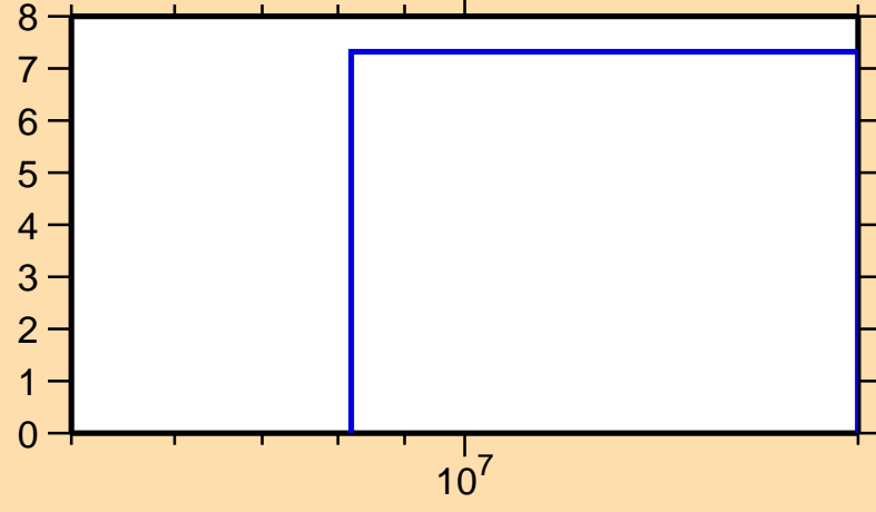
\Delta\sigma/\sigma vs. E for ^{199}\text{Bi}(n,\text{el.})
