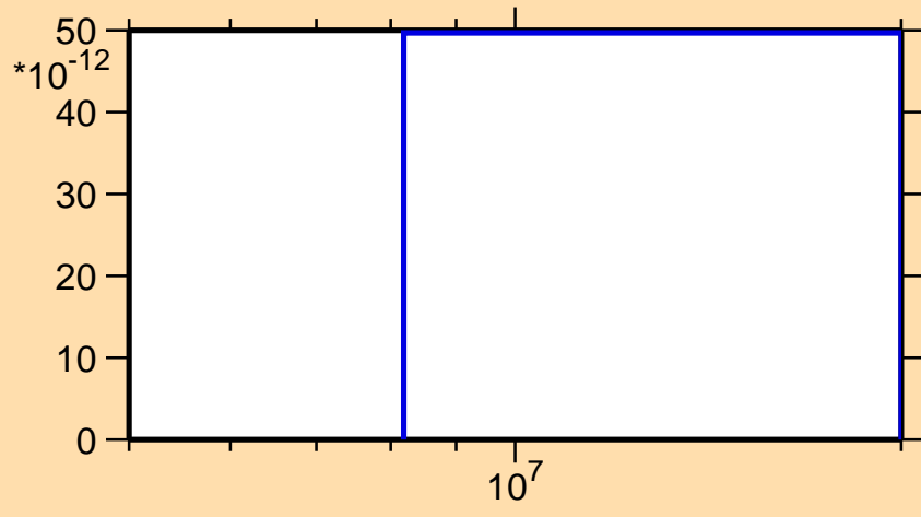
\sigma vs. E for ^{199}\text{Bi} (mt 45)
