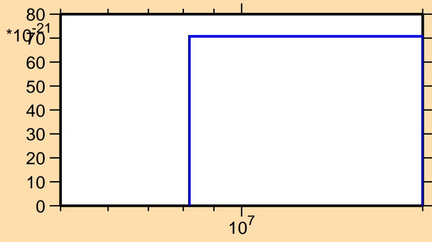
\sigma vs. E for ^{199}\text{Bi} (mt 42)
