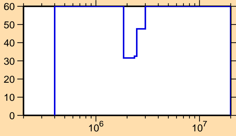
\Delta\sigma/\sigma vs. E for ^{199}\text{Bi}(n,n_1)
