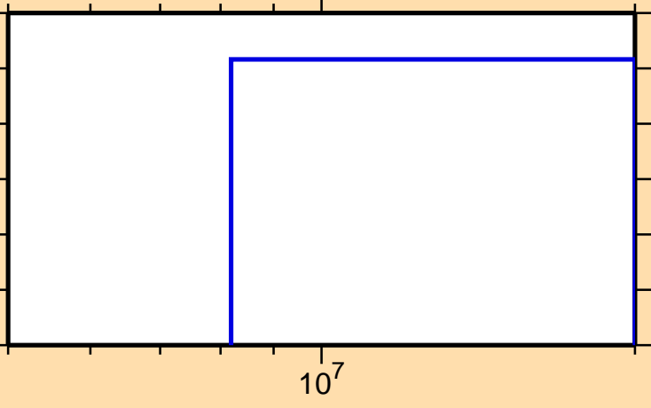
\sigma vs. E for ^{199}\text{Bi}(n,3n)
