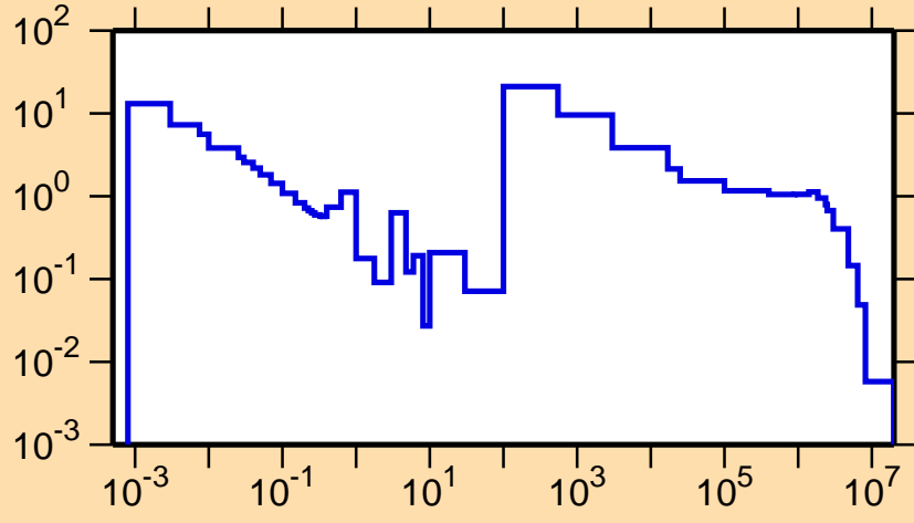
\sigma vs. E for ^{199}\text{Bi}(n,\gamma)
