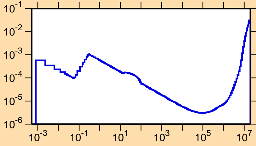
\sigma vs. E for ^{200}\text{Bi}(n,\alpha)
