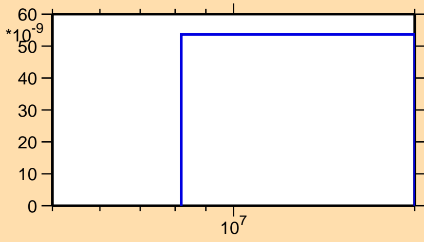
\sigma vs. E for ^{200}\text{Bi}(n,2n\alpha)
