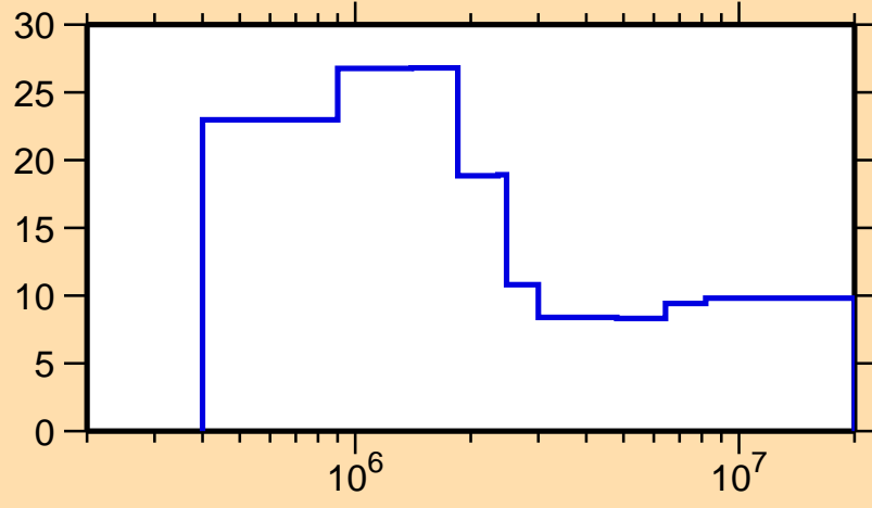
\Delta\sigma/\sigma vs. E for ^{200}\text{Bi}(n,n\text{nonel.})
