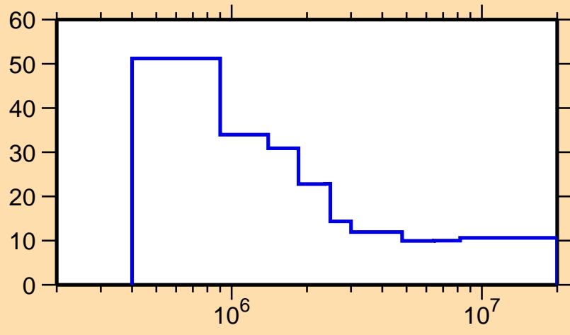
\Delta\sigma/\sigma vs. E for ^{200}\text{Bi}(n,n\text{cont.})
