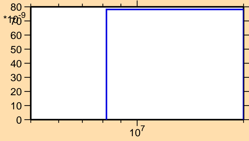
\sigma vs. E for ^{200}\text{Bi}(n,\text{nd})
