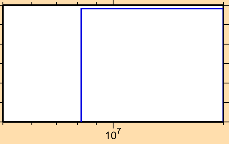
\sigma vs. E for ^{200}\text{Bi}(n,nt)
