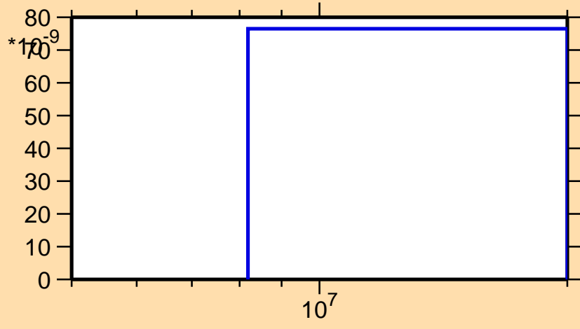
\sigma vs. E for ^{200}\text{Bi}(n,\text{He}3)
