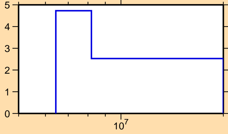
\Delta\sigma/\sigma vs. E for ^{200}\text{Bi}(n,\text{el.})
