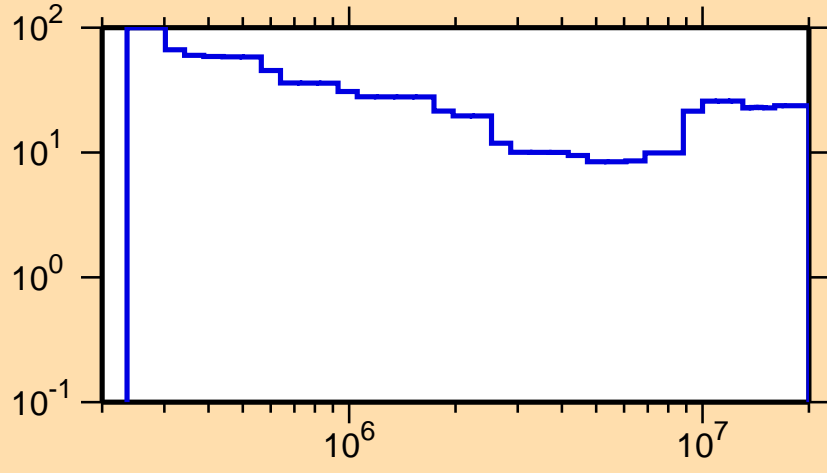
\Delta\sigma/\sigma vs. E for ^{200}\text{Bi}(n,n\text{cont.})
