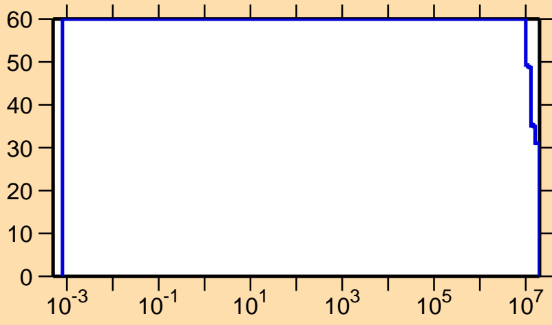
\Delta\sigma/\sigma vs. E for ^{200}\text{Bi}(n,p)
