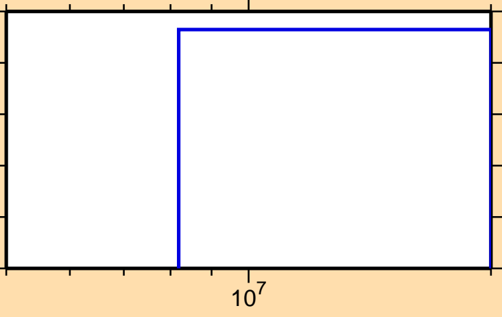
\sigma vs. E for ^{200}\text{Bi}(n,2np)
