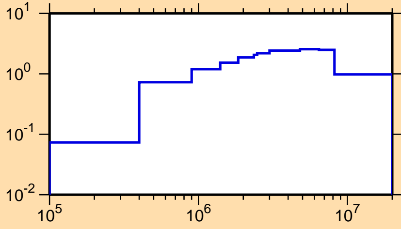
\sigma vs. E for ^{200}\text{Bi}(n,\text{inel.})
