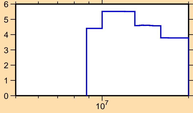
\Delta\sigma/\sigma vs. E for ^{201}\text{Bi}(n,\text{el.})
