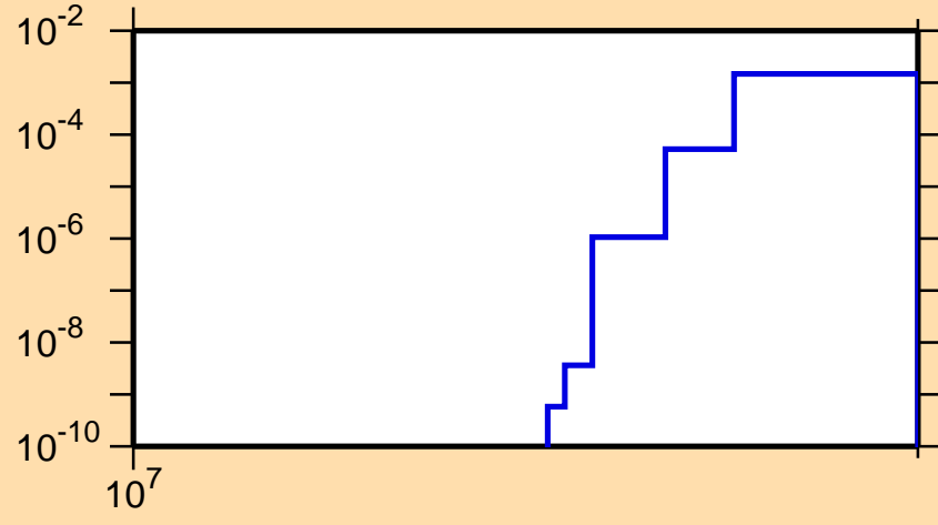
\sigma vs. E for ^{201}\text{Bi}(n,2np)
