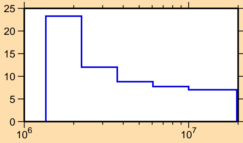
\Delta\sigma/\sigma vs. E for ^{201}\text{Bi}(n,n\text{onel.})
