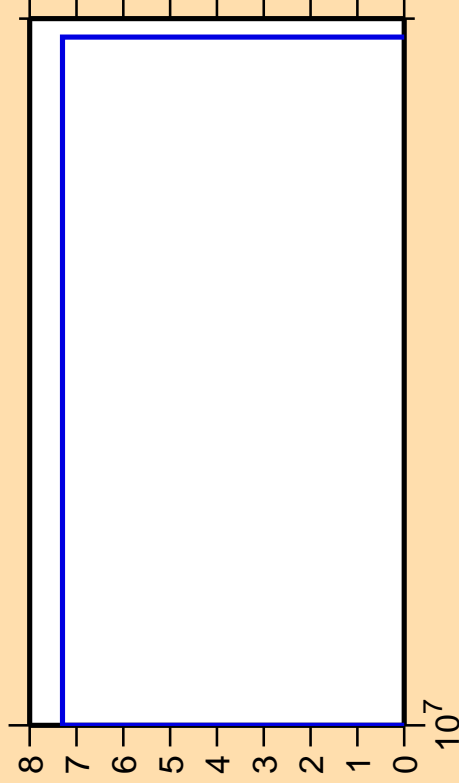
\Delta\sigma/\sigma vs. E for ^{201}\text{Bi} (mt 45)
