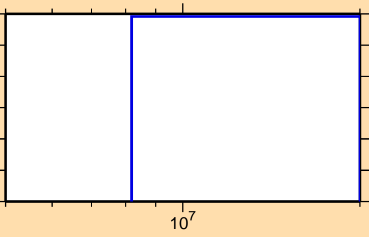
\sigma vs. E for ^{201}\text{Bi}(n,\text{He3})
