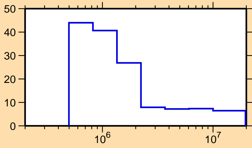
\Delta\sigma/\sigma vs. E for ^{202}\text{Bi}(n,n\text{onel.})
