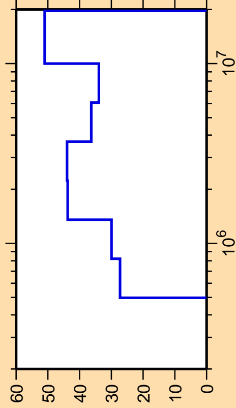
\Delta\sigma/\sigma vs. E for ^{202}\text{Bi}(n,n_4)
