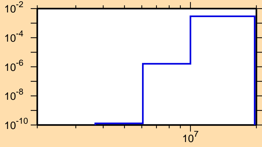
\sigma vs. E for ^{202}\text{Bi}(n,d)
