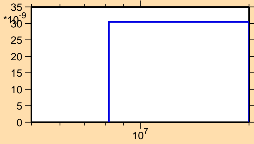
\sigma vs. E for ^{202}\text{Bi}(n,2n\alpha)
