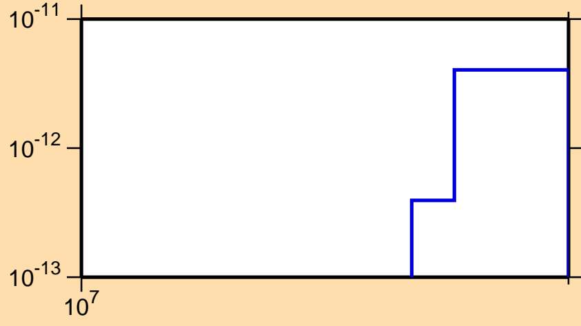
\sigma vs. E for ^{203}\text{Bi} (mt 45)
