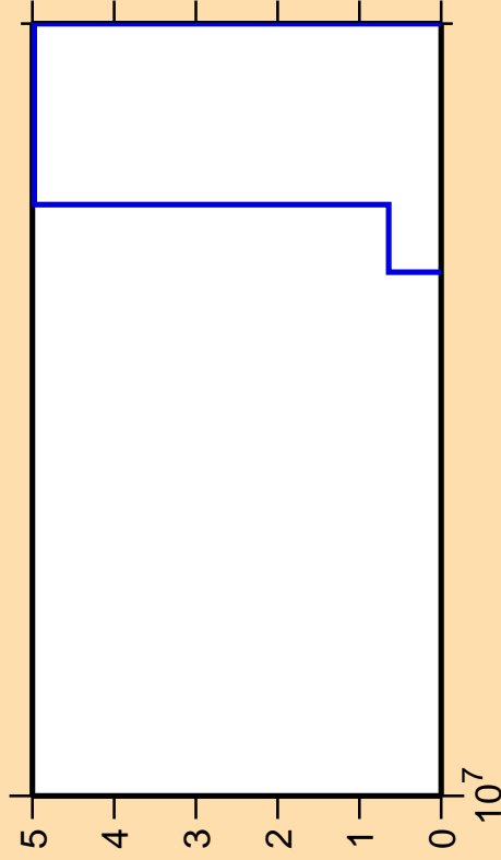
\Delta\sigma/\sigma vs. E for ^{203}\text{Bi}(\text{mt117})
