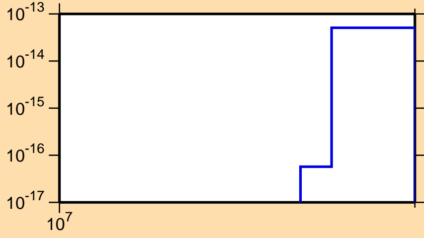
\sigma vs. E for ^{203}\text{Bi} (mt 34)
