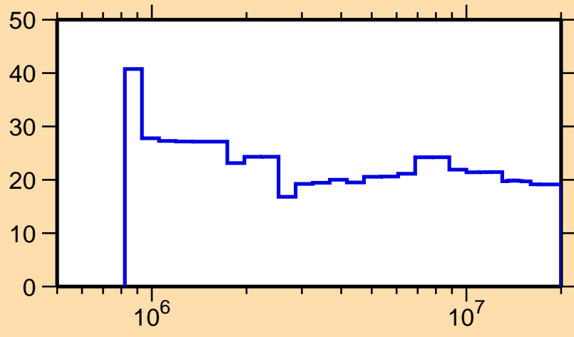
\Delta\sigma/\sigma vs. E for ^{203}\text{Bi}(n,n_1)
