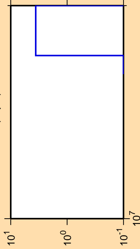
\Delta\sigma/\sigma vs. E for ^{203}\text{Bi}(n,\text{pd})
