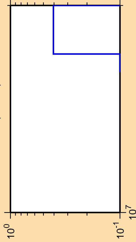
\Delta\sigma/\sigma vs. E for ^{203}\text{Bi} (mt 34)
