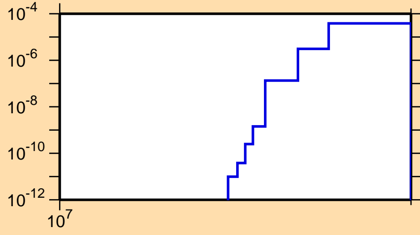
\sigma vs. E for ^{203}\text{Bi}(n,2np)
