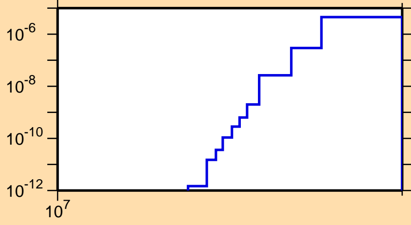
\sigma vs. E for ^{203}\text{Bi}(n,\text{nd})
