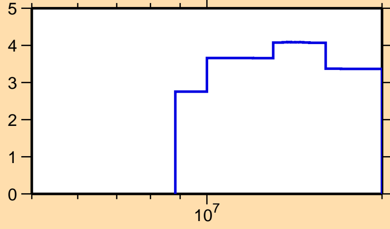
\Delta\sigma/\sigma vs. E for ^{203}\text{Bi}(n,\text{el.})
