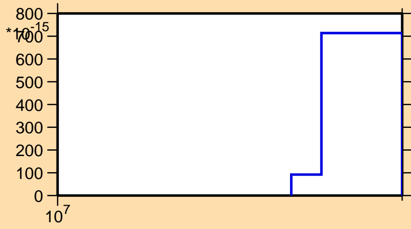
\sigma vs. E for ^{203}\text{Bi}(\text{mt117})
