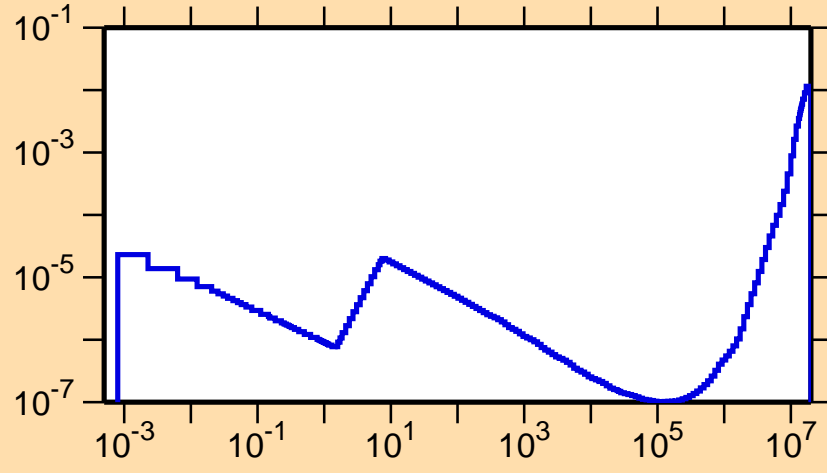
\sigma vs. E for ^{203}\text{Bi}(n,\alpha)
