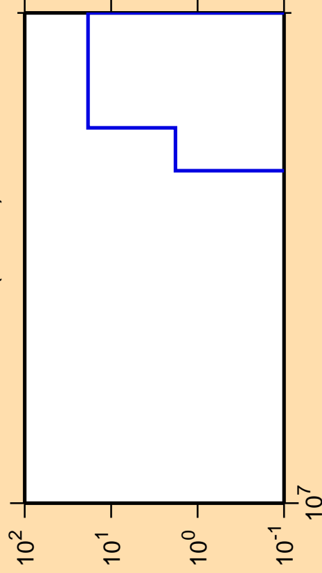
\Delta\sigma/\sigma vs. E for ^{203}\text{Bi} (mt 45)
