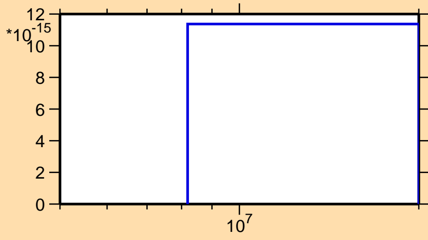
\sigma vs. E for ^{203}\text{Bi}(\text{mt117})
