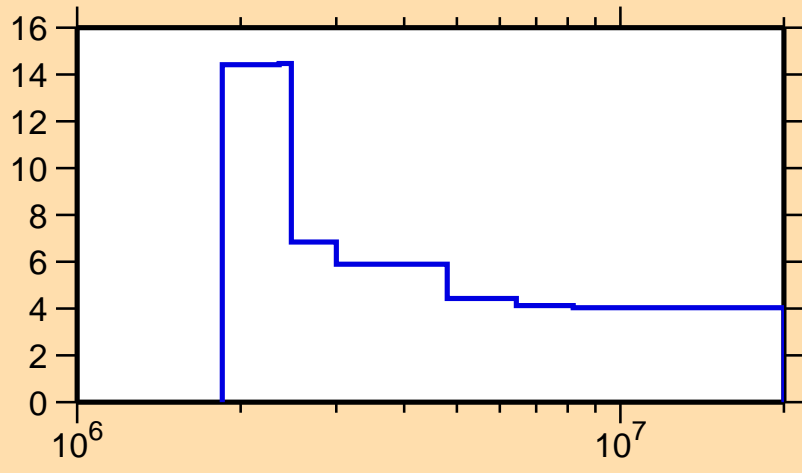
\Delta\sigma/\sigma vs. E for ^{203}\text{Bi}(n,n\text{nonel.})
