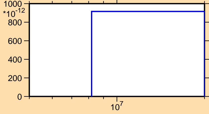
\sigma vs. E for ^{203}\text{Bi}(n,p\alpha)
