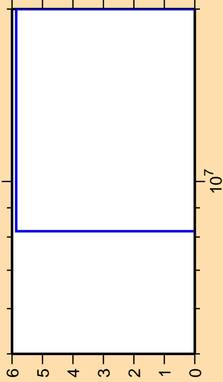
\Delta\sigma/\sigma vs. E for ^{203}\text{Bi}(n,2n)
