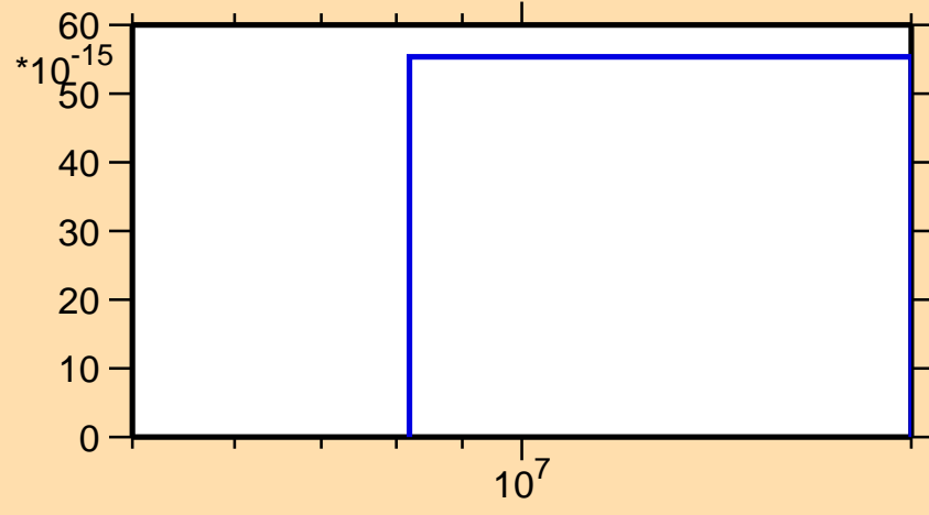
\sigma vs. E for ^{203}\text{Bi} (mt 45)
