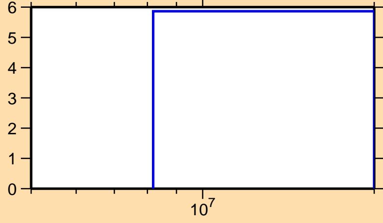
\Delta\sigma/\sigma vs. E for ^{203}\text{Bi}(n,2n)
