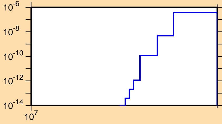
\sigma vs. E for ^{204}\text{Bi}(n,nt)
