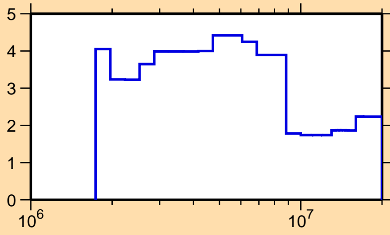
\Delta\sigma/\sigma vs. E for ^{204}\text{Bi}(n,\text{tot.})
