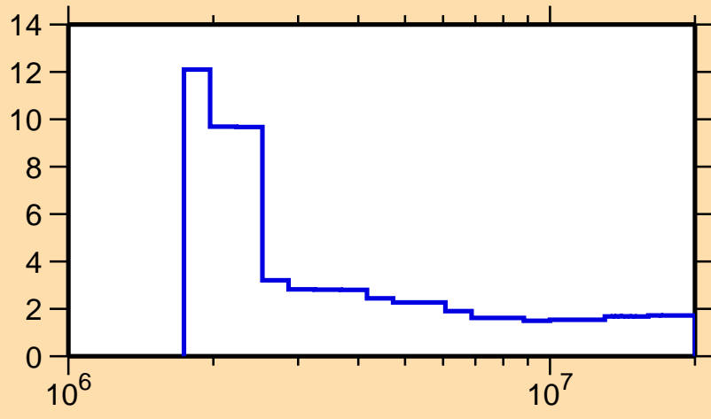
\Delta\sigma/\sigma vs. E for ^{204}\text{Bi}(n,\text{nonel.})
