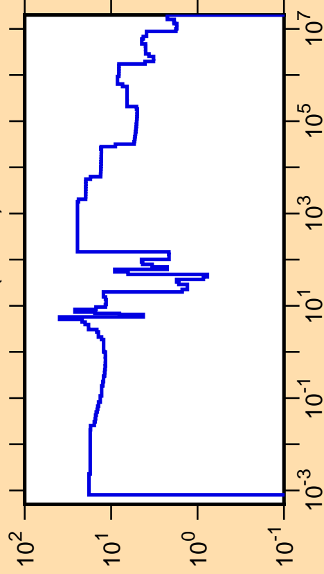
\Delta\sigma/\sigma vs. E for ^{204}\text{Bi}(n,\text{tot.})
