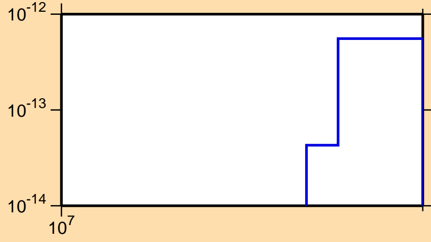
\sigma vs. E for ^{204}\text{Bi} (mt 45)
