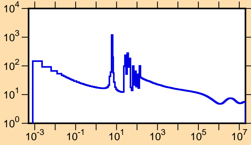
\sigma vs. E for ^{204}\text{Bi}(n,\text{tot.})
