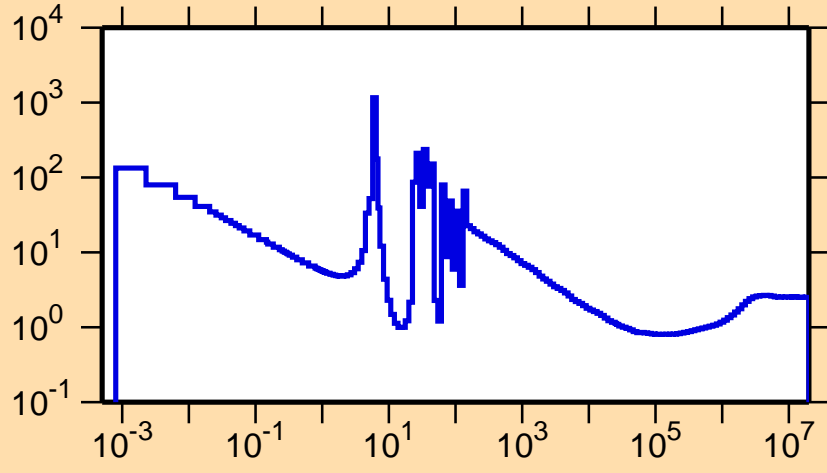
\sigma vs. E for ^{204}\text{Bi}(n,\text{nonel.})
