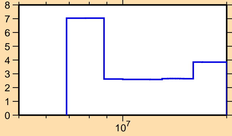
\Delta\sigma/\sigma vs. E for ^{204}\text{Bi}(n,\text{el.})
