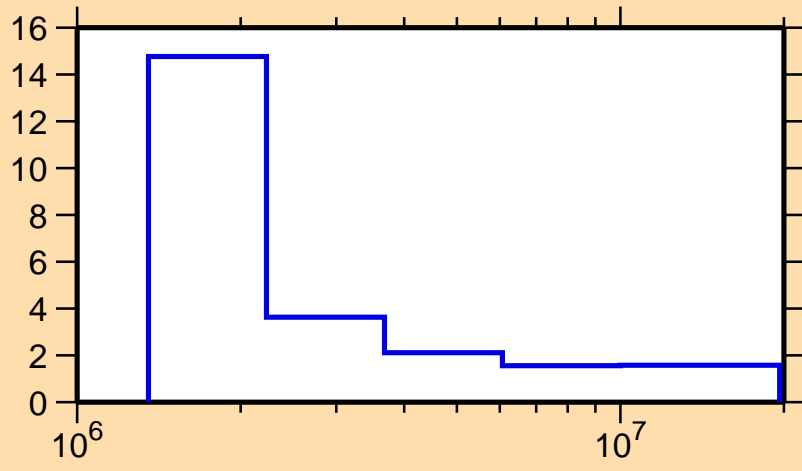
\Delta\sigma/\sigma vs. E for ^{204}\text{Bi}(n,n\text{onel.})
