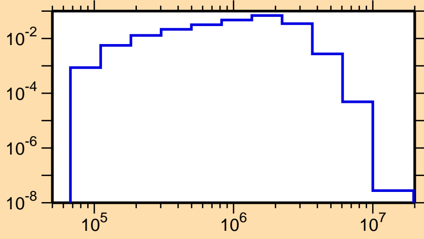
\sigma vs. E for ^{204}\text{Bi}(n,n_4)
