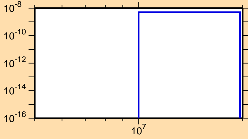
\sigma vs. E for ^{204}\text{Bi}(n,\text{He3})
