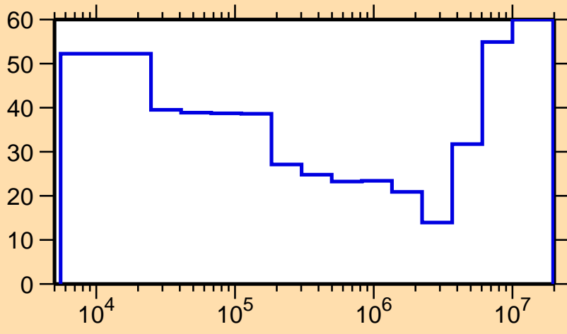
\Delta\sigma/\sigma vs. E for ^{204}\text{Bi}(n,n_1)
