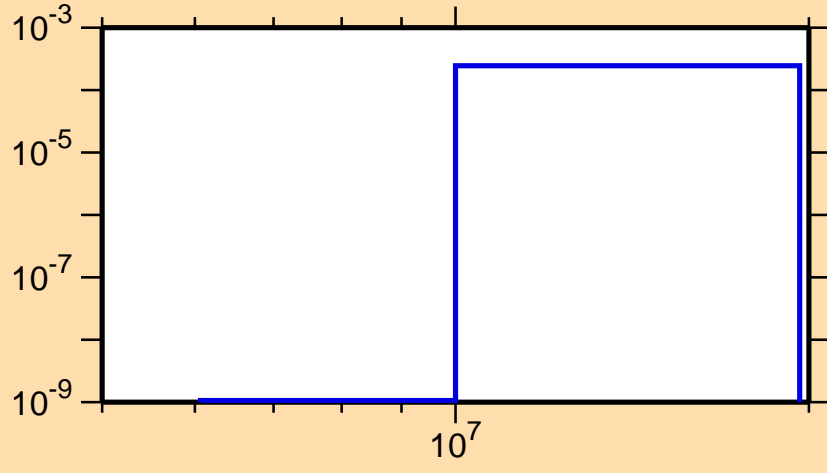
\sigma vs. E for ^{204}\text{Bi}(n,t)
