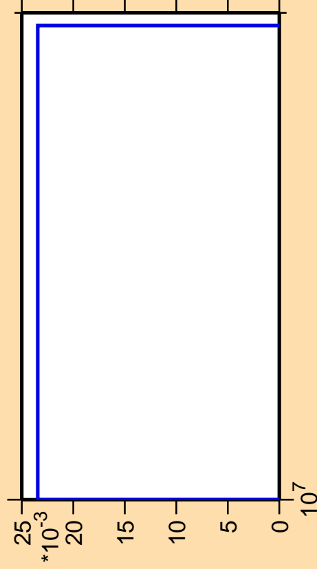
\Delta\sigma/\sigma vs. E for ^{204}\text{Bi}(\text{mt117})
