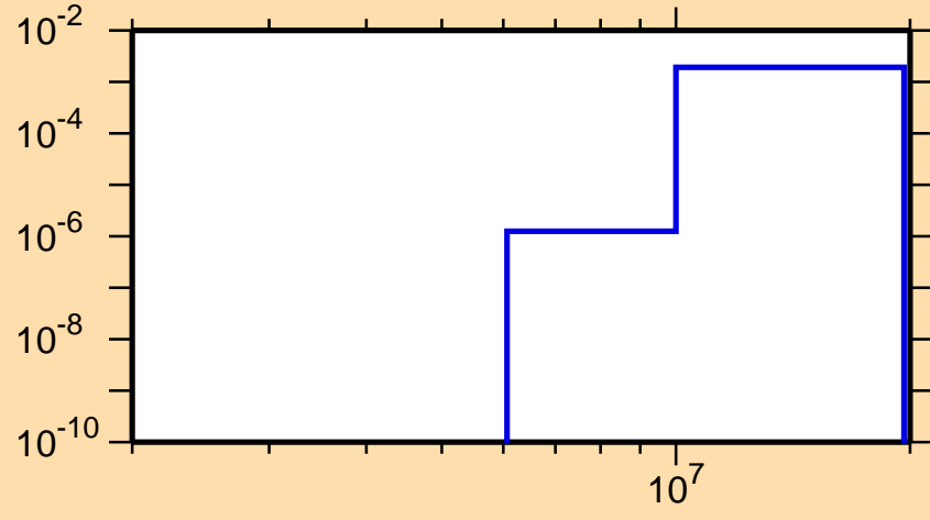
\sigma vs. E for ^{204}\text{Bi}(n,d)
