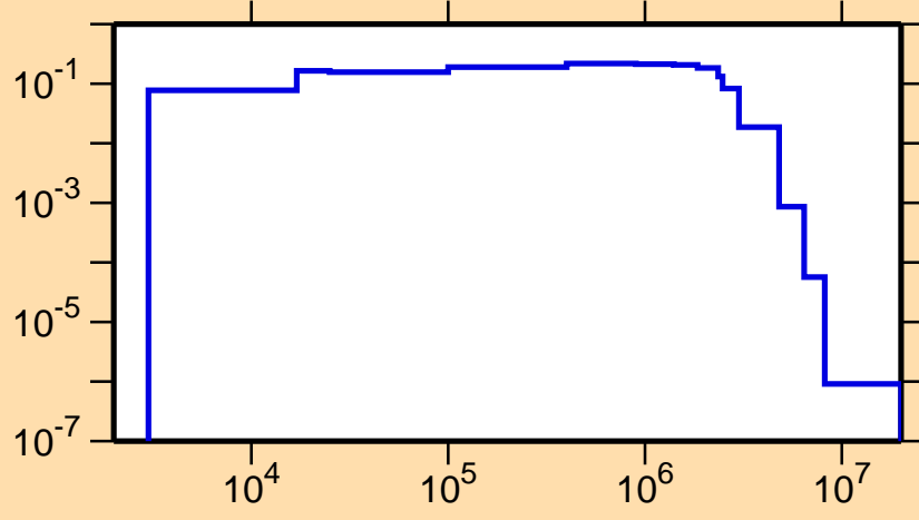
\sigma vs. E for ^{204}\text{Bi}(n,n_1)
