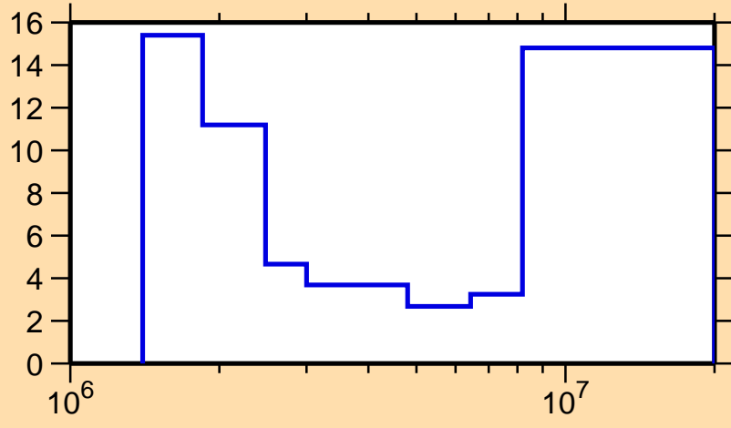
\Delta\sigma/\sigma vs. E for ^{204}\text{Bi}(n,ncont.)
