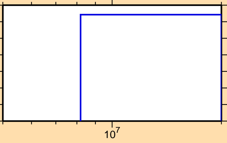
\sigma vs. E for ^{204}\text{Bi}(n,2n\alpha)
