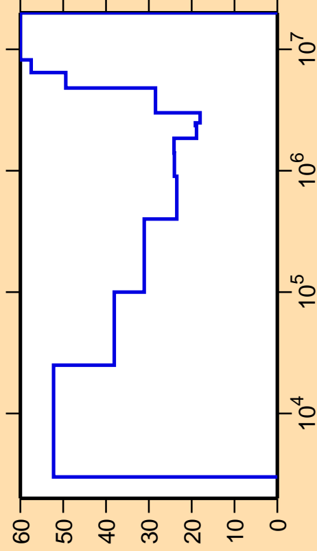
\Delta\sigma/\sigma vs. E for ^{204}\text{Bi}(n,n_1)
