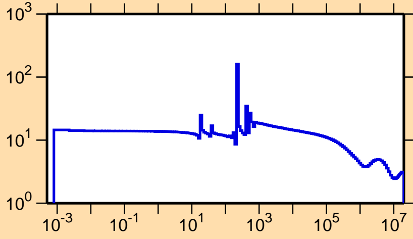
\sigma vs. E for ^{205}\text{Bi}(n,\text{el.})
