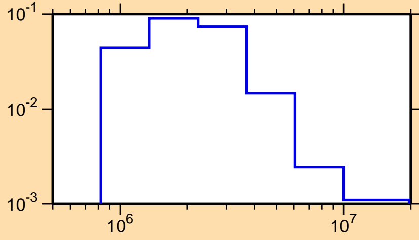
\sigma vs. E for ^{205}\text{Bi}(n,n_3)
