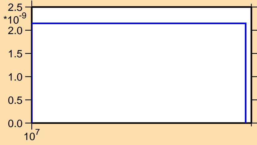
\sigma vs. E for ^{205}\text{Bi}(n,nt)
