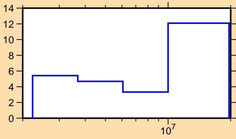
\Delta\sigma/\sigma vs. E for ^{205}\text{Bi}(n,ncont.)
