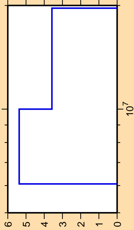
\Delta\sigma/\sigma vs. E for ^{205}\text{Bi}(n,2n)
