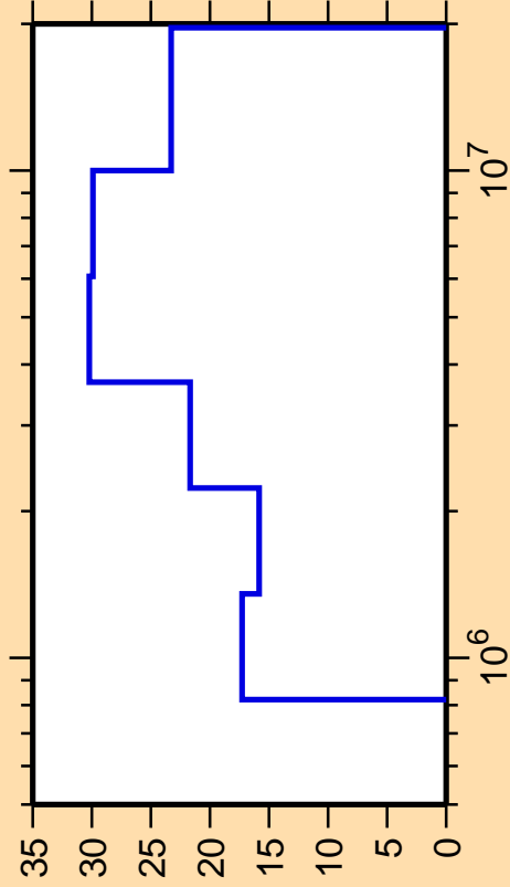
\Delta\sigma/\sigma vs. E for ^{205}\text{Bi}(n,n_4)
