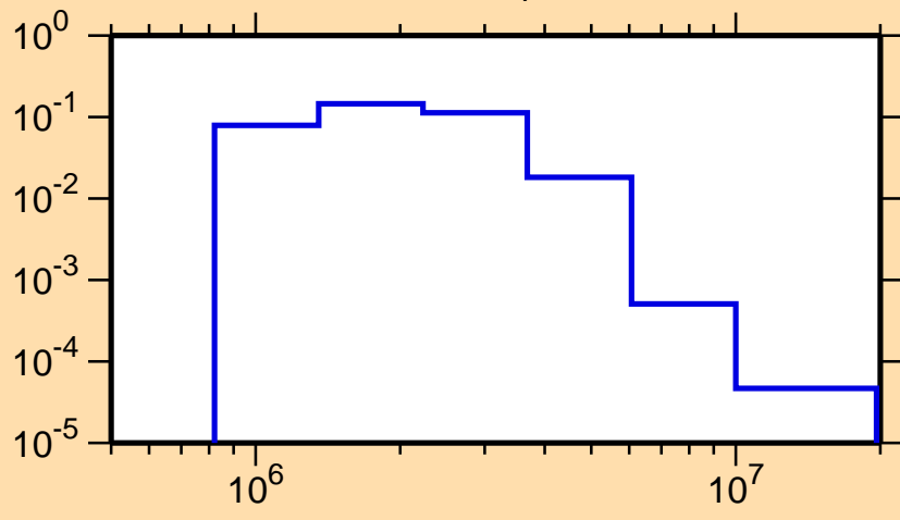
\sigma vs. E for ^{205}\text{Bi}(n,n_4)
