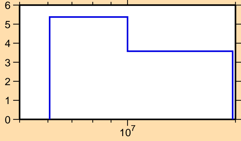
\Delta\sigma/\sigma vs. E for ^{205}\text{Bi}(n,2n)
