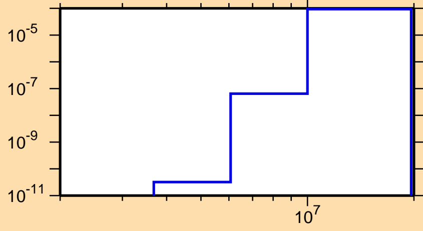
\sigma vs. E for ^{205}\text{Bi}(n,n\alpha)
