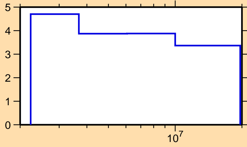
\Delta\sigma/\sigma vs. E for ^{205}\text{Bi}(n,n\text{nonel.})
