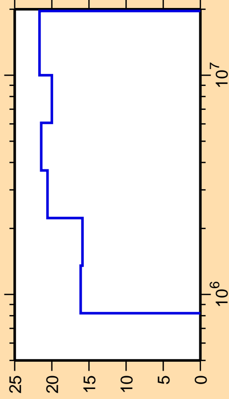
\Delta\sigma/\sigma vs. E for ^{205}\text{Bi}(n,n_3)
