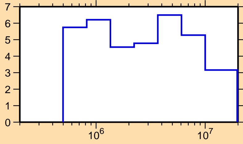
\Delta\sigma/\sigma vs. E for ^{205}\text{Bi}(n,\text{el.})
