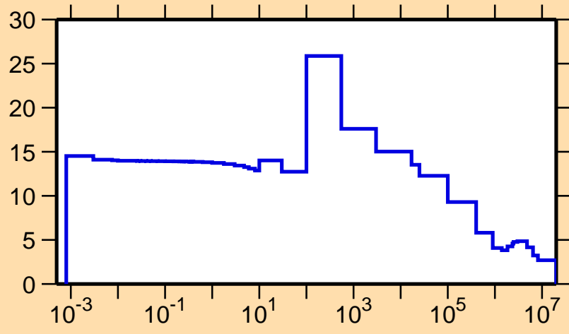
\sigma vs. E for ^{205}\text{Bi}(n,\text{el.})
