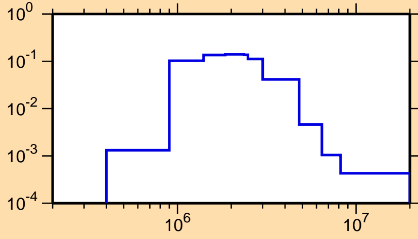
\sigma vs. E for ^{205}\text{Bi}(n,n_2)
