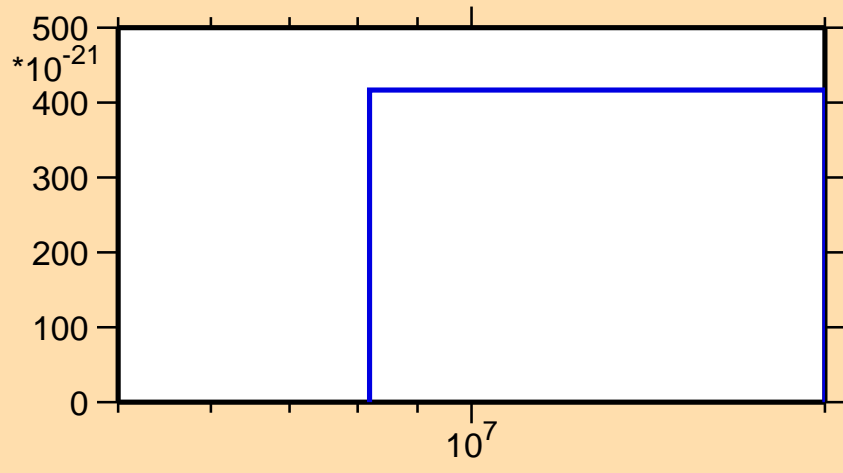
\sigma vs. E for ^{205}\text{Bi} (mt 42)
