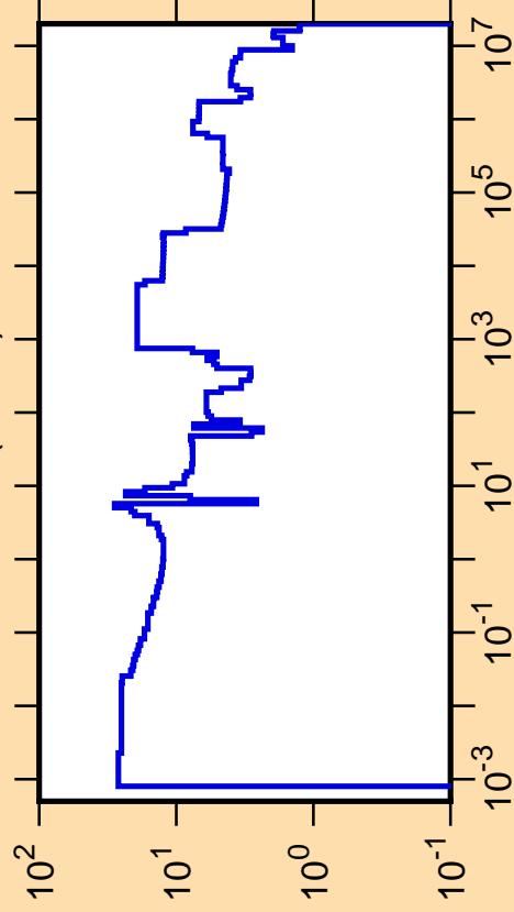
\Delta\sigma/\sigma vs. E for ^{206}\text{Bi}(n,\text{tot.})
