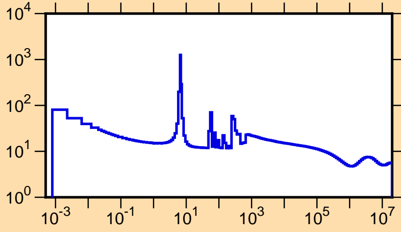
\sigma vs. E for ^{206}\text{Bi}(n,\text{tot.})
