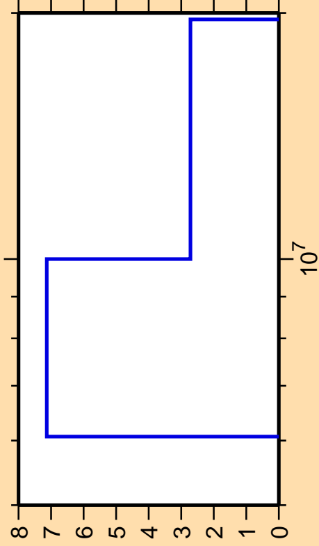
\Delta\sigma/\sigma vs. E for ^{206}\text{Bi}(n,2n)
