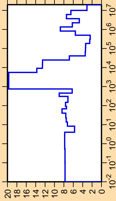
\Delta\sigma/\sigma vs. E for ^{206}\text{Bi}(n,\text{el.})
