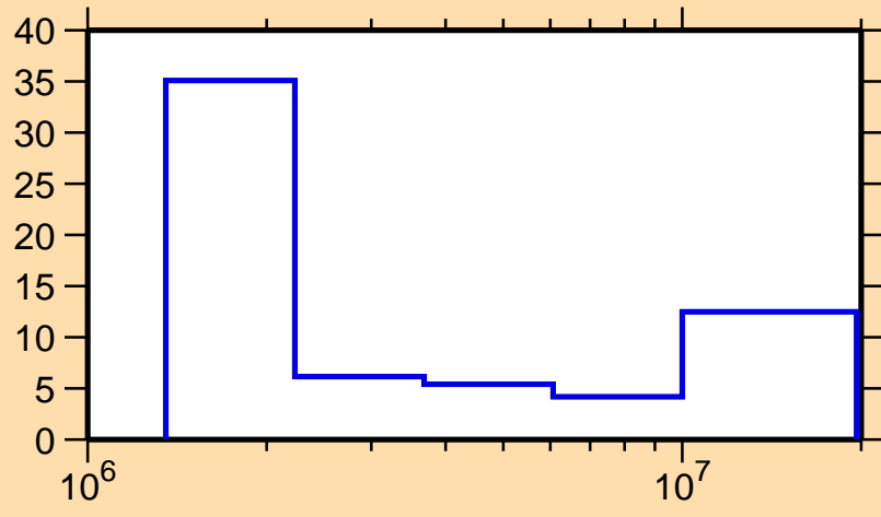
\Delta\sigma/\sigma vs. E for ^{206}\text{Bi}(n,n\text{cont.})
