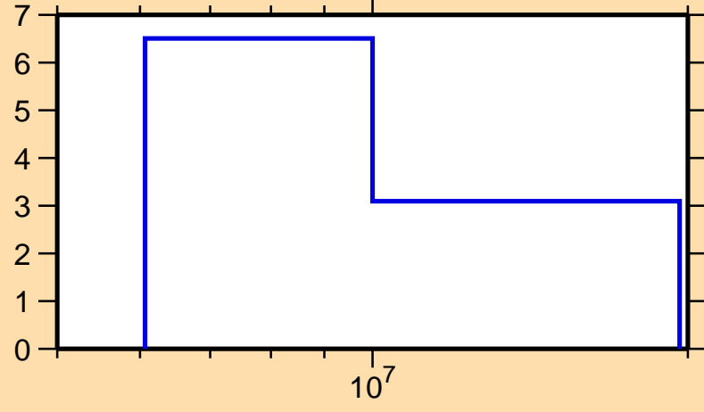
\Delta\sigma/\sigma vs. E for ^{206}\text{Bi}(n,\text{el.})
