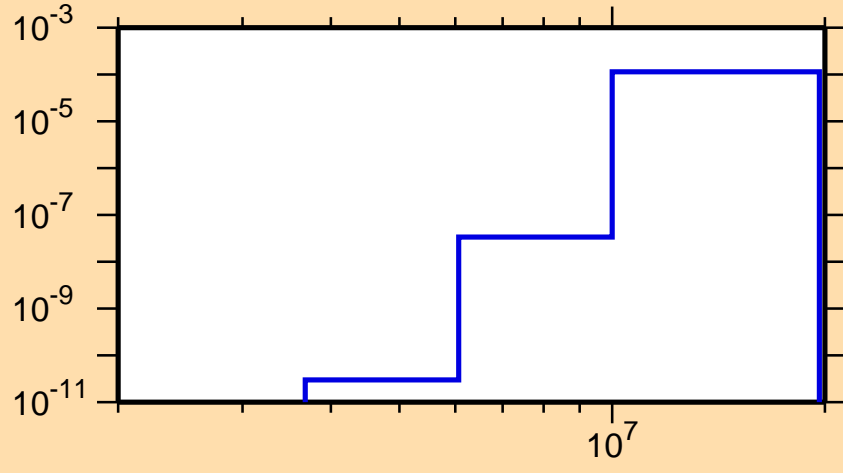
\sigma vs. E for ^{206}\text{Bi}(n,n\alpha)
