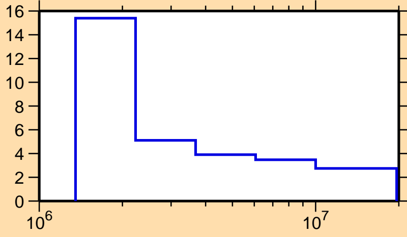
\Delta\sigma/\sigma vs. E for ^{206}\text{Bi}(n,n\text{onel.})
