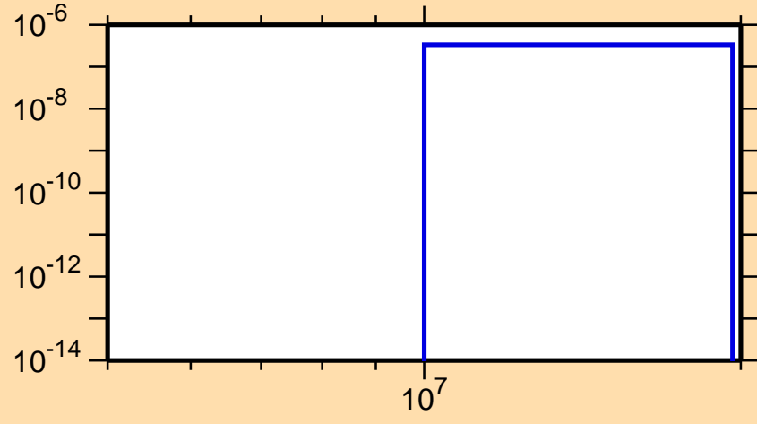
\sigma vs. E for ^{206}\text{Bi}(n,\text{nd})
