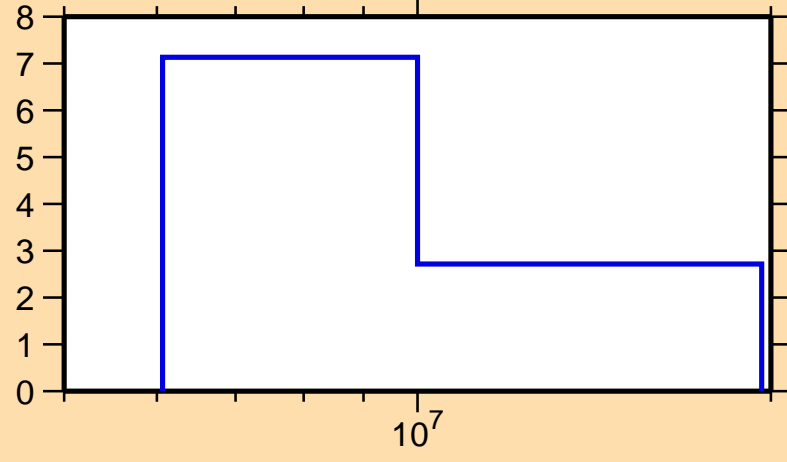
\Delta\sigma/\sigma vs. E for ^{206}\text{Bi}(n,2n)
