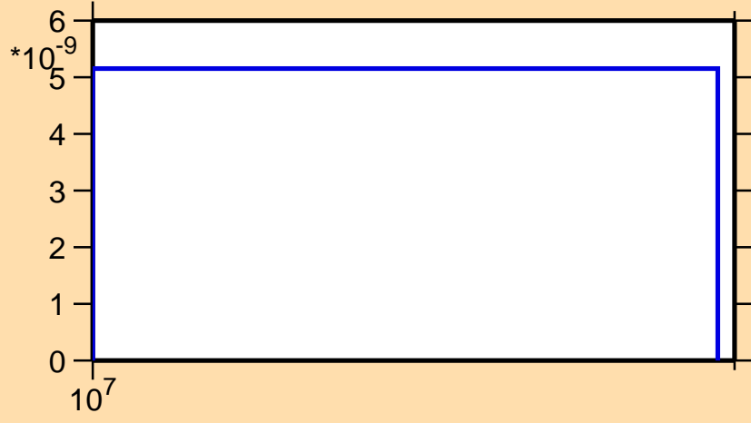
\sigma vs. E for ^{206}\text{Bi}(n,nt)
