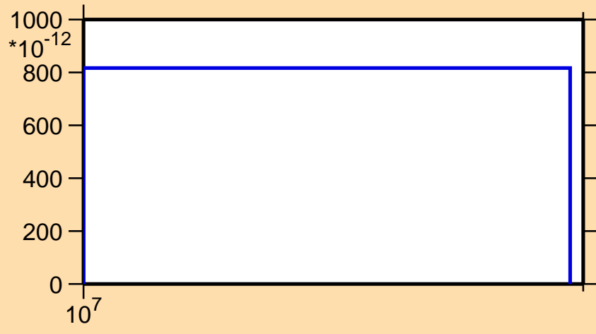
\sigma vs. E for ^{206}\text{Bi}(n,\text{He}3)
