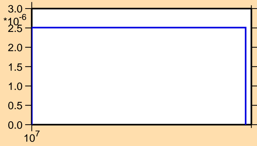
\sigma vs. E for ^{206}\text{Bi}(n,2np)
