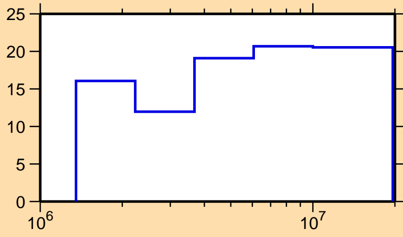
\Delta\sigma/\sigma vs. E for ^{206}\text{Bi}(n,n_1)
