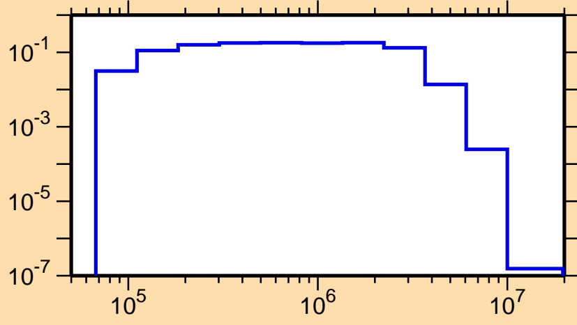
\sigma vs. E for ^{206}\text{Bi}(n,n_3)
