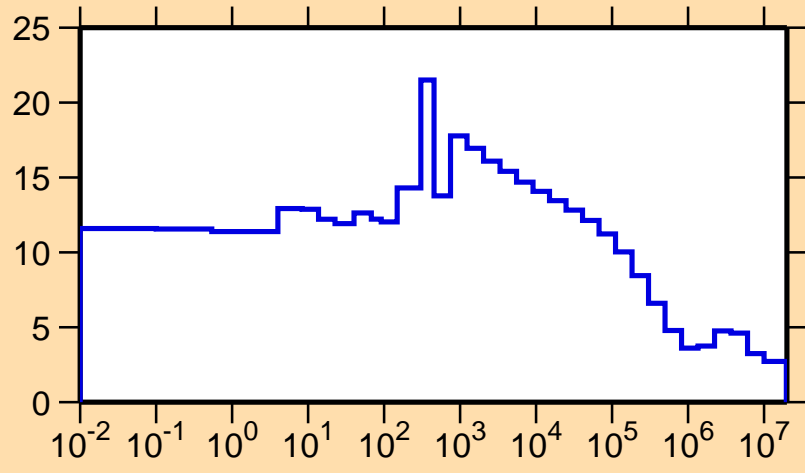
\sigma vs. E for ^{206}\text{Bi}(n,\text{el.})
