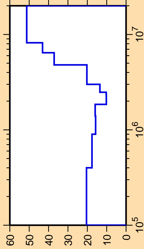
\Delta\sigma/\sigma vs. E for ^{206}\text{Bi}(n,n_4)
