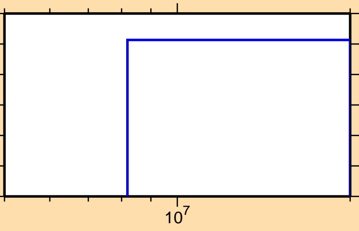
\sigma vs. E for ^{206}\text{Bi}(n,2n\alpha)
