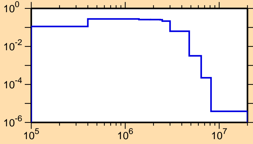
\sigma vs. E for ^{206}\text{Bi}(n,n_4)
