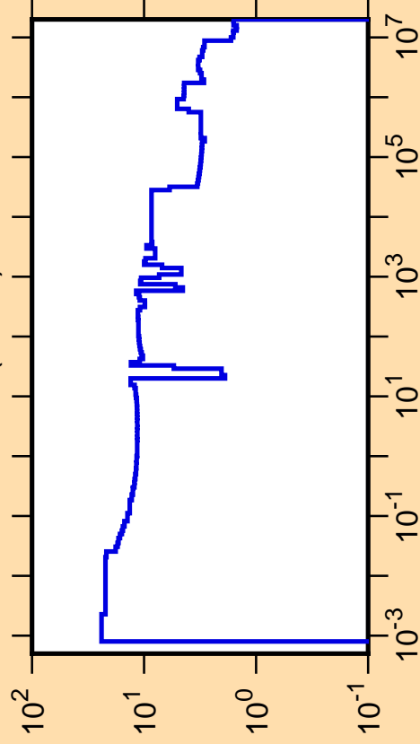
\Delta\sigma/\sigma vs. E for ^{207}\text{Bi}(n,\text{tot.})
