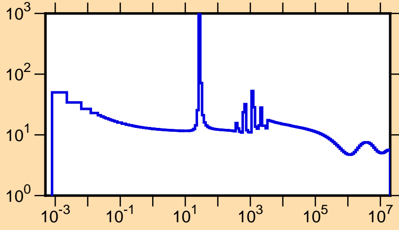
\sigma vs. E for ^{207}\text{Bi}(n,\text{tot.})
