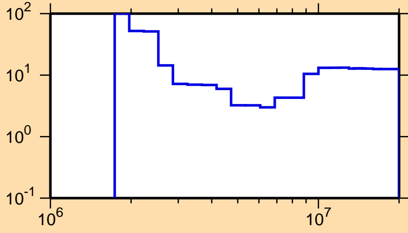
\Delta\sigma/\sigma vs. E for ^{207}\text{Bi}(n,n\text{cont.})
