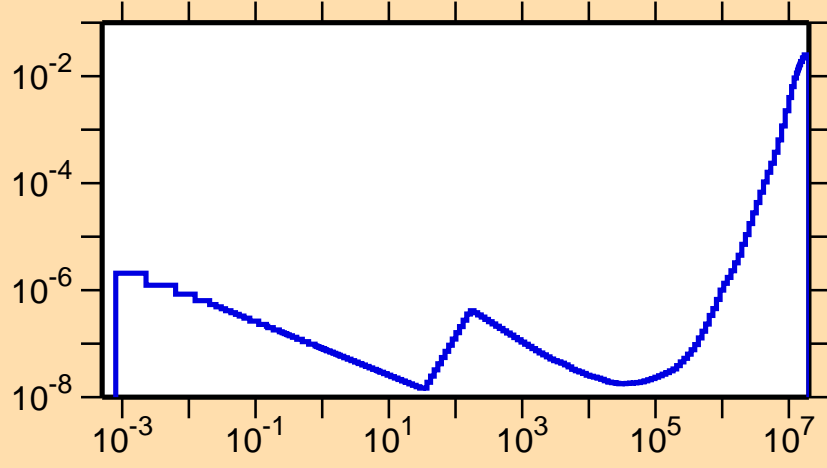
\sigma vs. E for ^{207}\text{Bi}(n,p)
