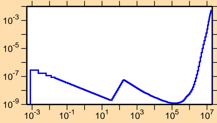
\sigma vs. E for ^{207}\text{Bi}(n,\alpha)
