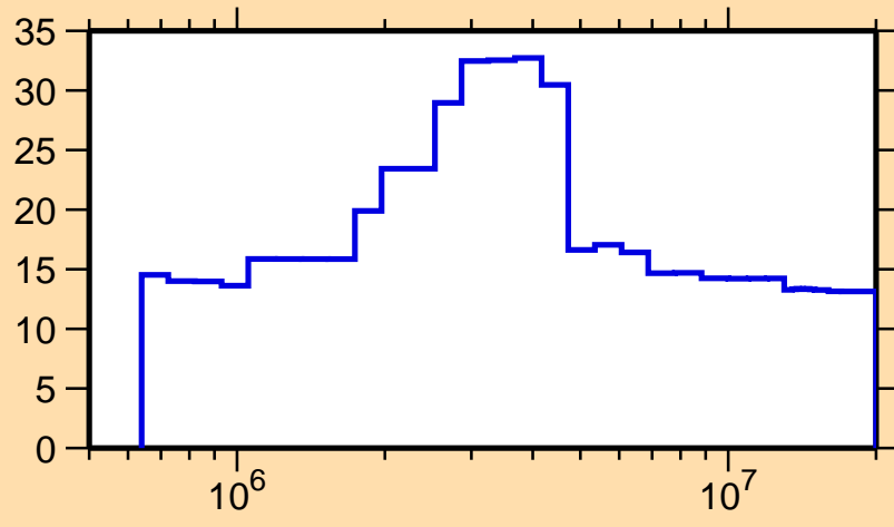
\Delta\sigma/\sigma vs. E for ^{207}\text{Bi}(n,n_1)
