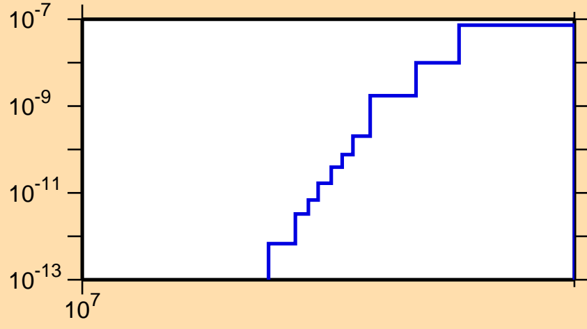
\sigma vs. E for ^{207}\text{Bi}(n,2n\alpha)
