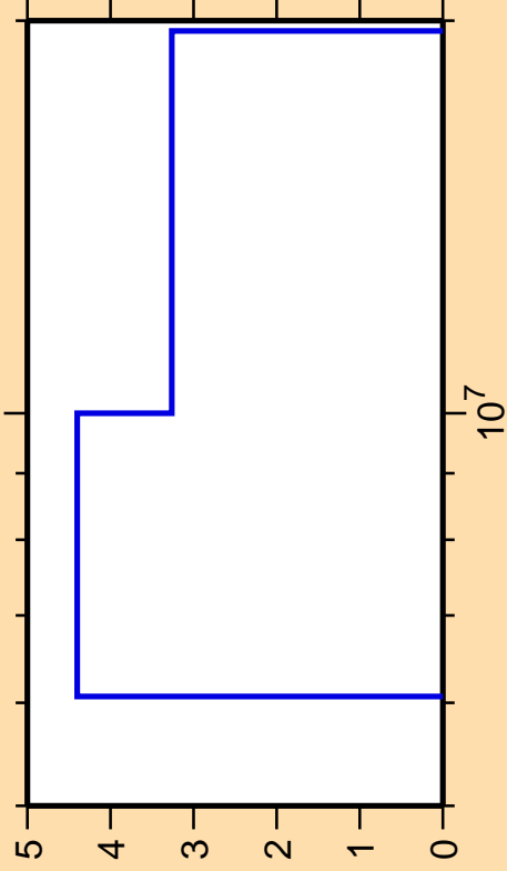
\Delta\sigma/\sigma vs. E for ^{207}\text{Bi}(n,2n)
