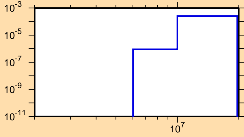
\sigma vs. E for ^{207}\text{Bi}(n,n\alpha)
