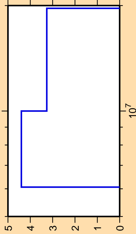
\Delta\sigma/\sigma vs. E for ^{207}\text{Bi}(n,2n)
