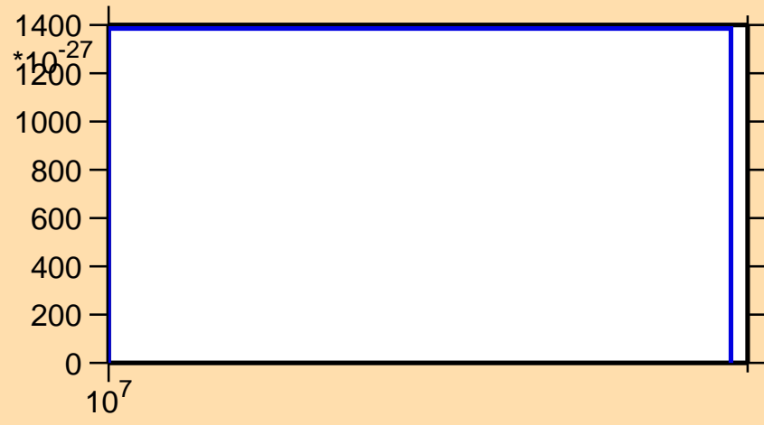
\sigma vs. E for ^{207}\text{Bi} (mt 42)
