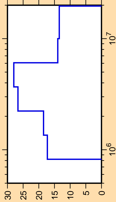
\Delta\sigma/\sigma vs. E for ^{207}\text{Bi}(n,n_4)
