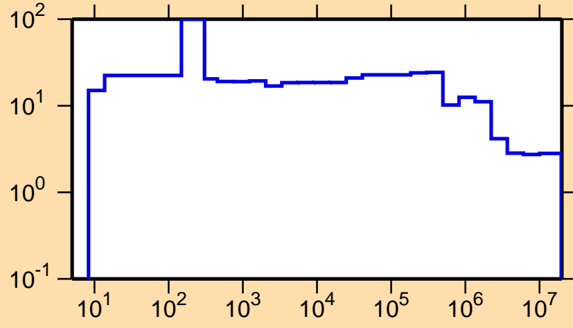
\Delta\sigma/\sigma vs. E for ^{207}\text{Bi}(n,\text{nonel.})
