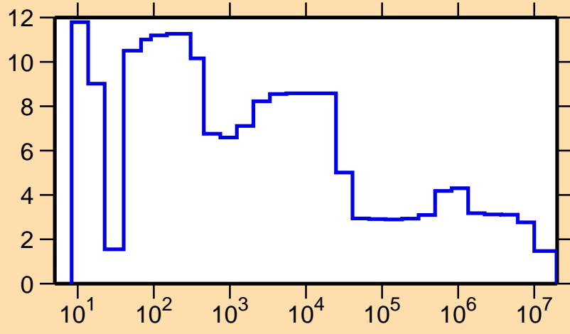
\Delta\sigma/\sigma vs. E for ^{207}\text{Bi}(n,\text{tot.})
