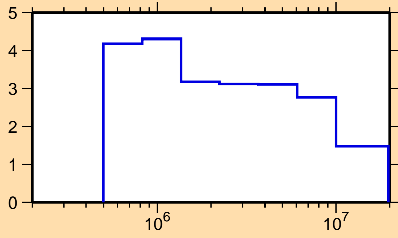
\Delta\sigma/\sigma vs. E for ^{207}\text{Bi}(n,\text{tot.})
