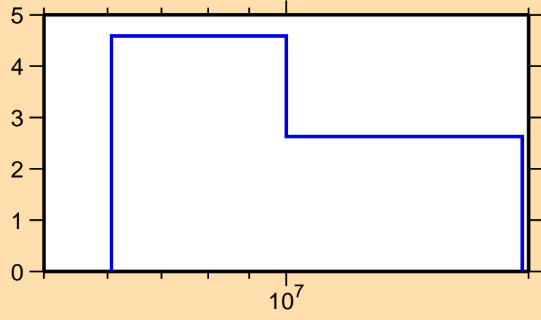
\Delta\sigma/\sigma vs. E for ^{207}\text{Bi}(n,\text{el.})
