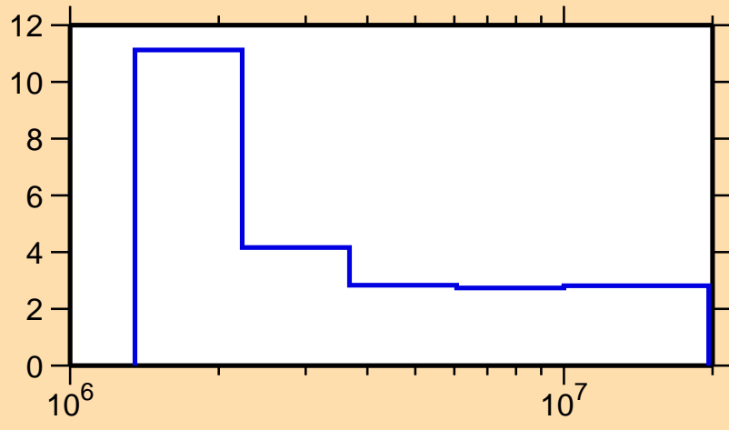
\Delta\sigma/\sigma vs. E for ^{207}\text{Bi}(n,n\text{onel.})
