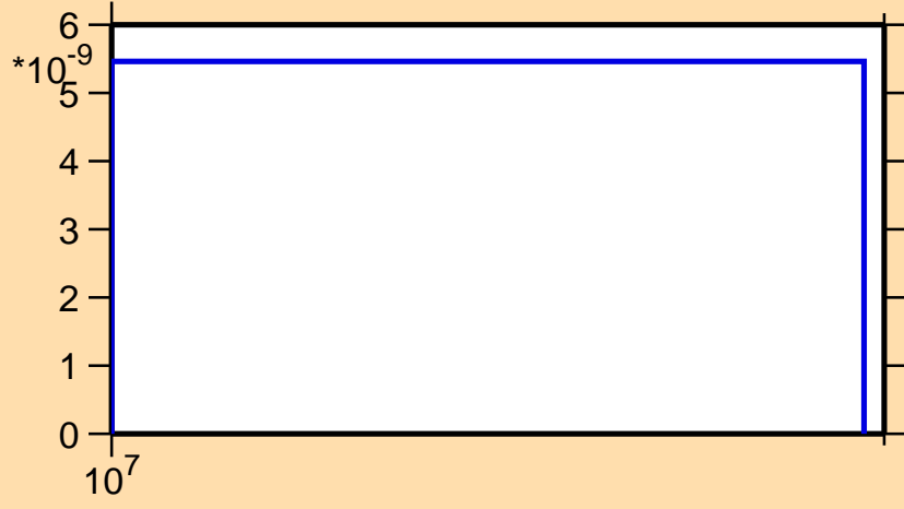
\sigma vs. E for ^{207}\text{Bi}(n,nt)
