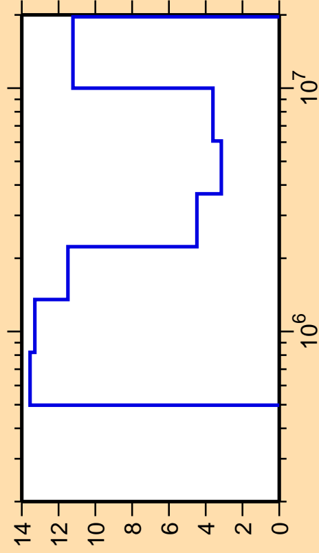
\Delta\sigma/\sigma vs. E for ^{207}\text{Bi}(n,\text{inel.})
