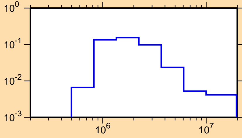
\sigma vs. E for ^{207}\text{Bi}(n,n_2)
