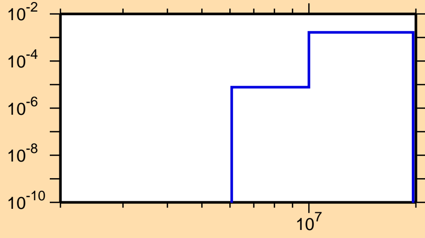
\sigma vs. E for ^{207}\text{Bi}(n,np)
