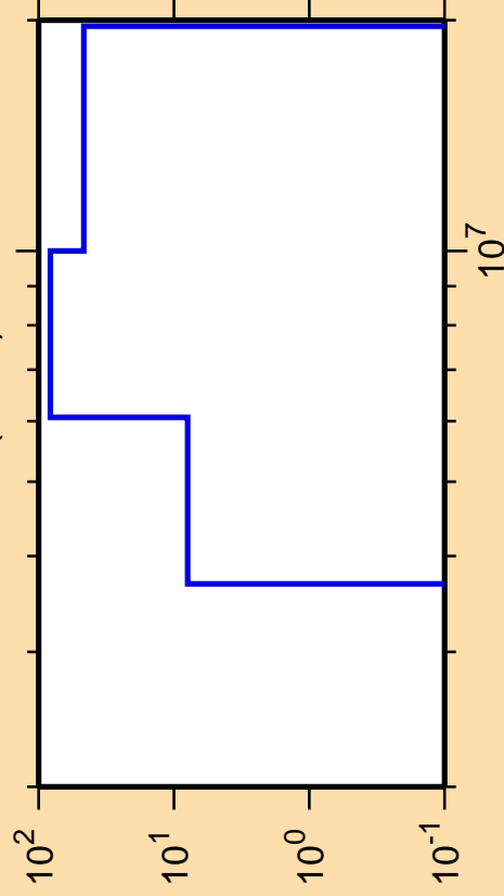
\Delta\sigma/\sigma vs. E for ^{207}\text{Bi}(n,n\alpha)
