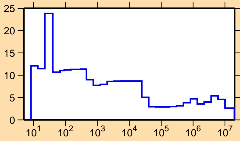
\Delta\sigma/\sigma vs. E for ^{207}\text{Bi}(n,\text{el.})
