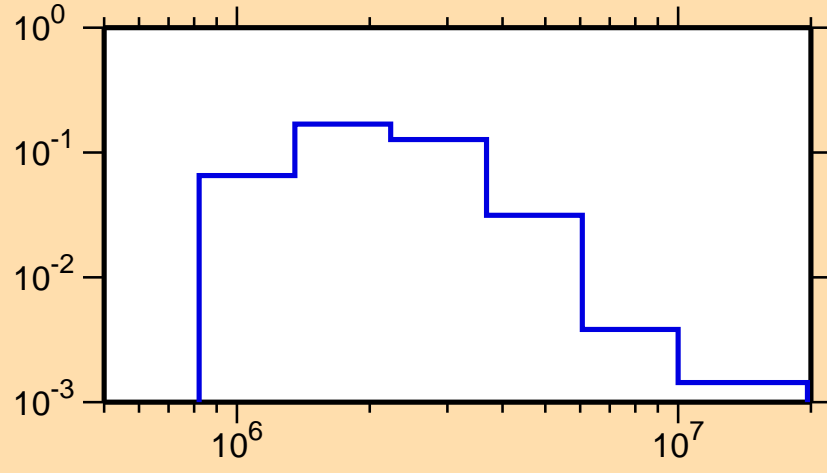
\sigma vs. E for ^{207}\text{Bi}(n,n_4)
