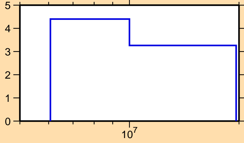
\Delta\sigma/\sigma vs. E for ^{207}\text{Bi}(n,2n)
