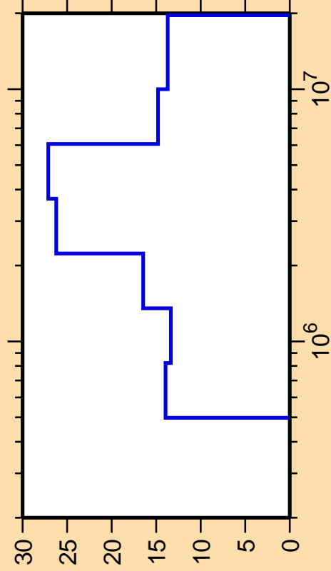
\Delta\sigma/\sigma vs. E for ^{207}\text{Bi}(n,n_2)
