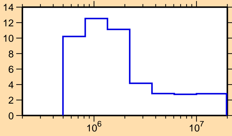
\Delta\sigma/\sigma vs. E for ^{207}\text{Bi}(n,\text{nonel.})
