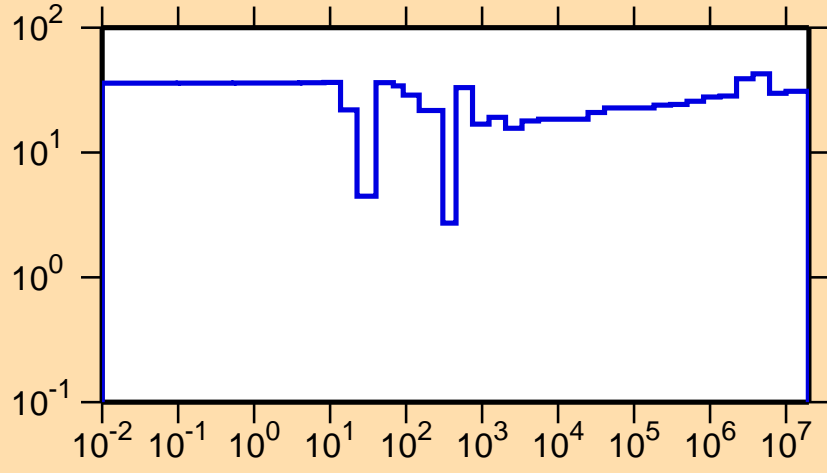
\Delta\sigma/\sigma vs. E for ^{207}\text{Bi}(n,\gamma)
