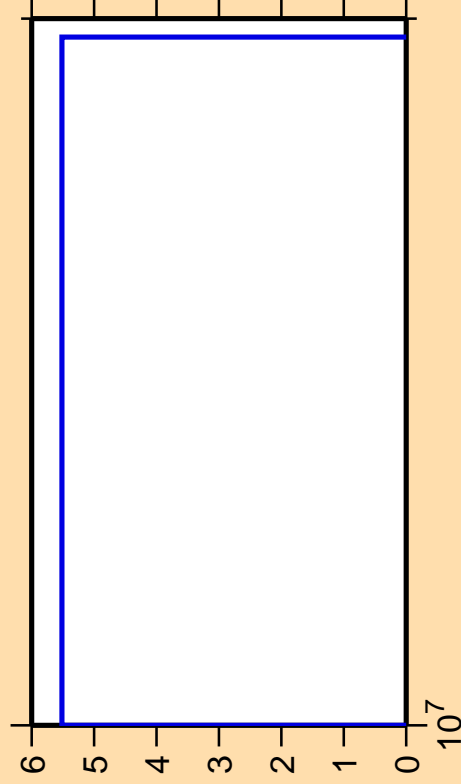
\Delta\sigma/\sigma vs. E for ^{207}\text{Bi}(n,3n)
