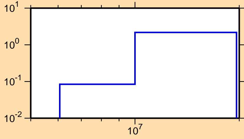
\sigma vs. E for ^{207}\text{Bi}(n,2n)
