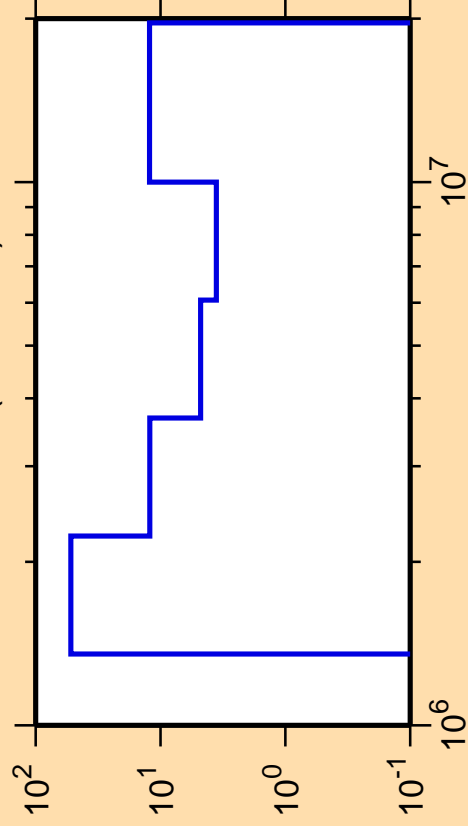
\Delta\sigma/\sigma vs. E for ^{207}\text{Bi}(n,\text{ncont.})
