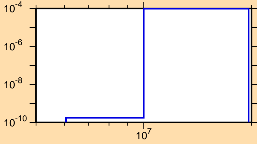
\sigma vs. E for ^{207}\text{Bi}(n,t)
