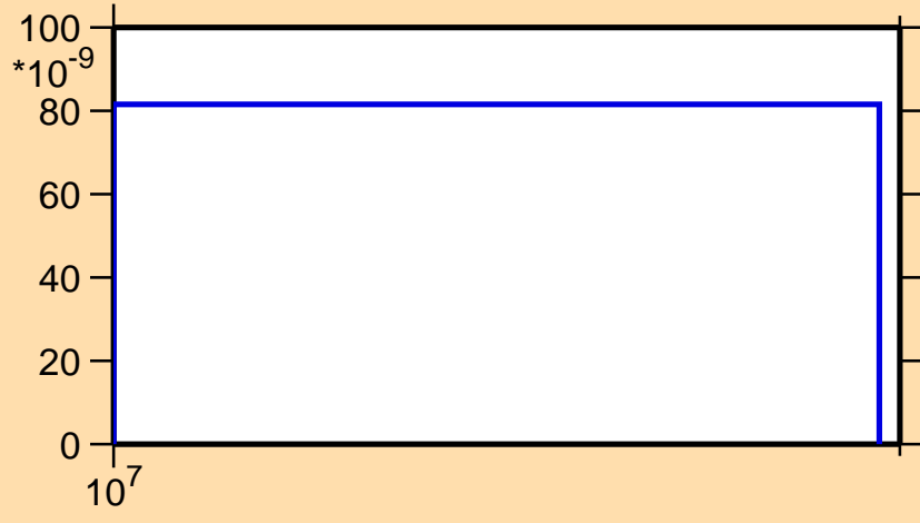
\sigma vs. E for ^{207}\text{Bi}(n,\text{nd})
