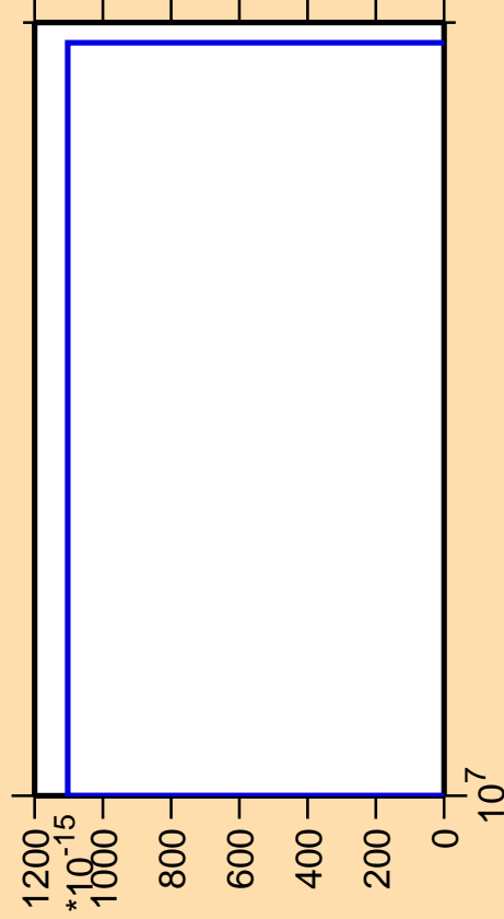
\Delta\sigma/\sigma vs. E for ^{207}\text{Bi} (mt 42)
