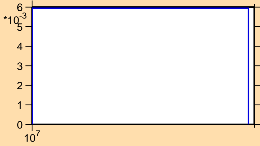
\sigma vs. E for ^{207}\text{Bi}(n,3n)
